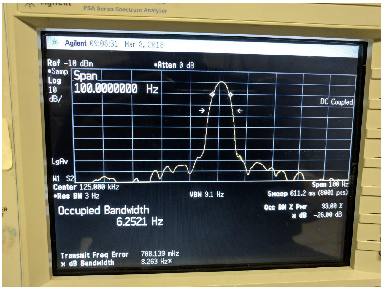
125kHz CW Signal
