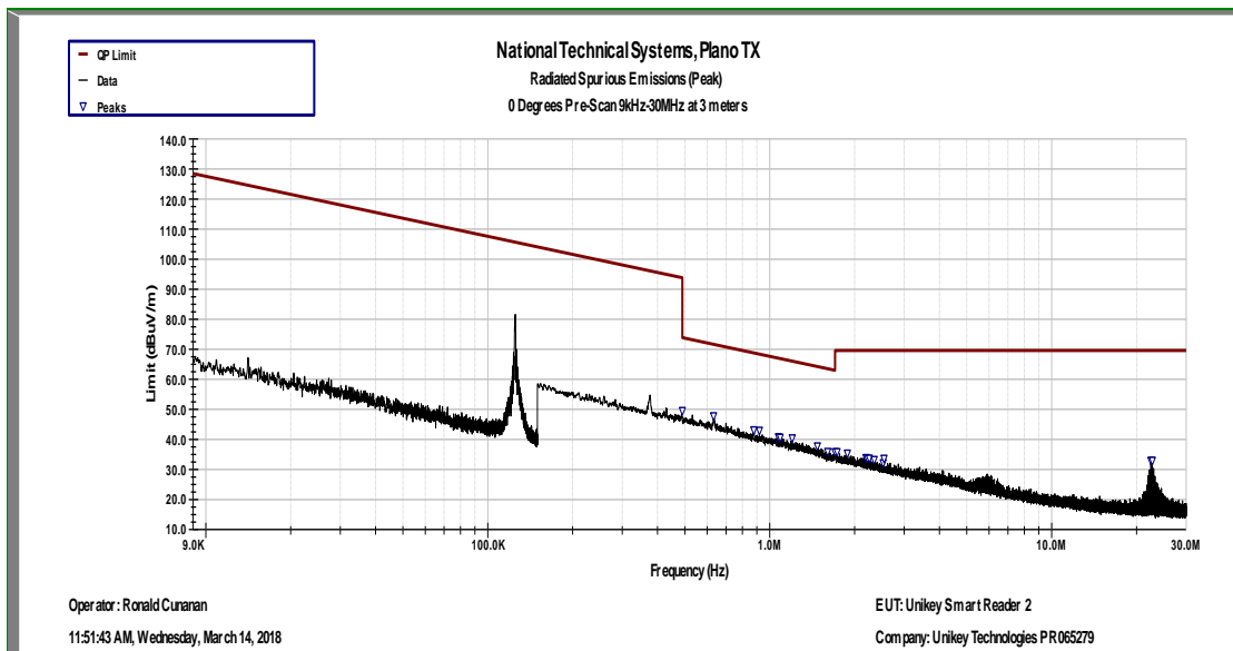
Radiated Spurious Emissions 9k-30MHz - Parallel
