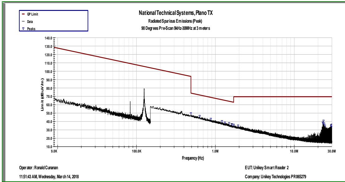
Radiated Spurious Emissions 9k-30MHz – Perpendicular
