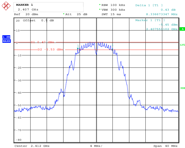
802.11b Low Channel
