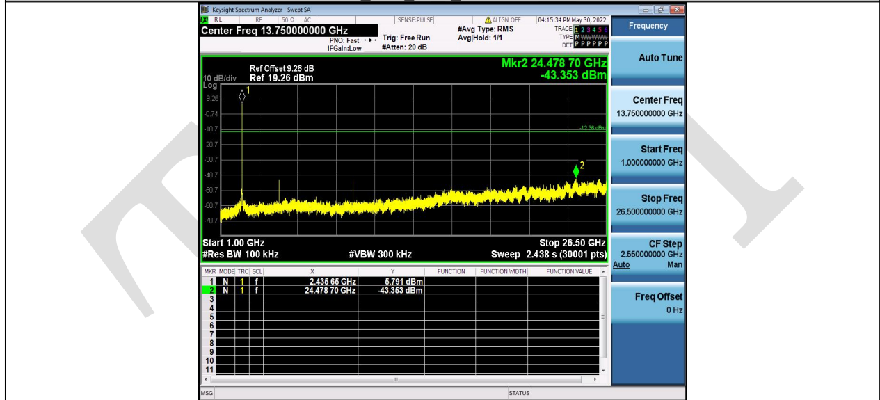
11B Ant1_2462_0~Reference
