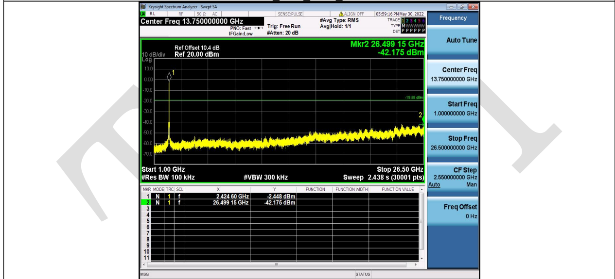
11N40SISO_Ant1_2437_0~Reference
