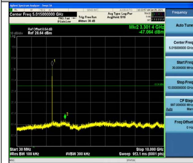
Spurious emission(2437MHz)
