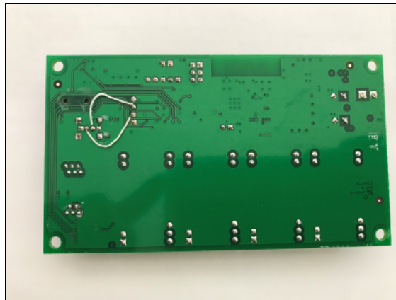
Figure 2: PCB – Back
