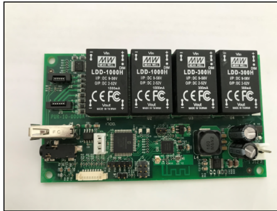
Figure 1: PCB – Front Note: PCB antenna shown is not being used
