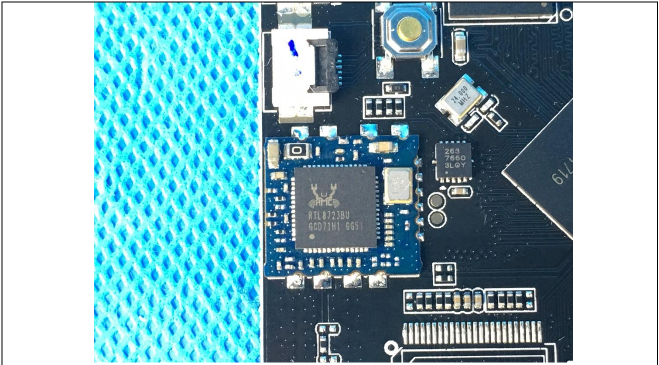
Details of: PCB Transmitter Module view 1
