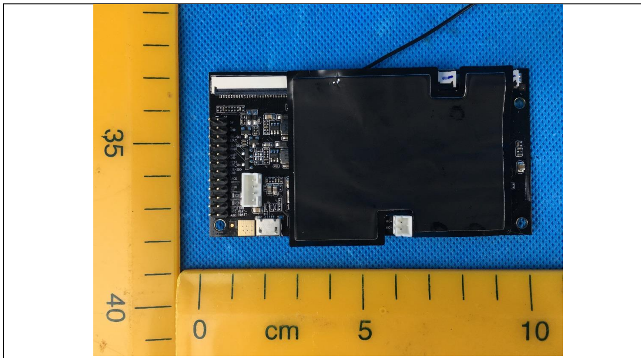
Details of: PCB view 7
