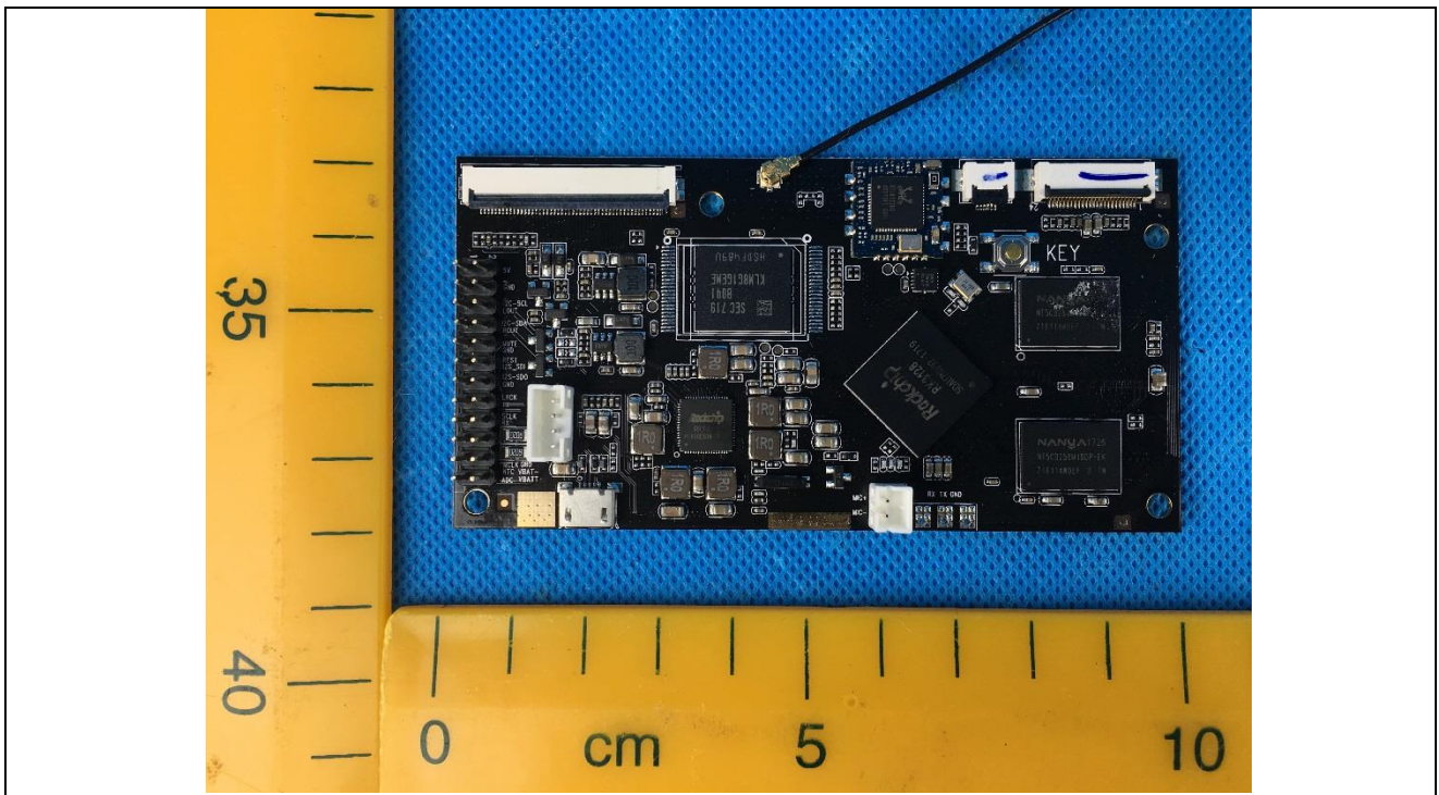
Details of: PCB view 8
