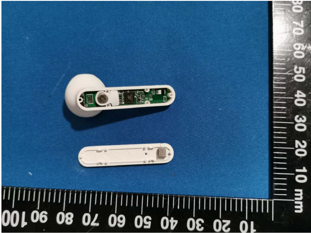
Right Unit
