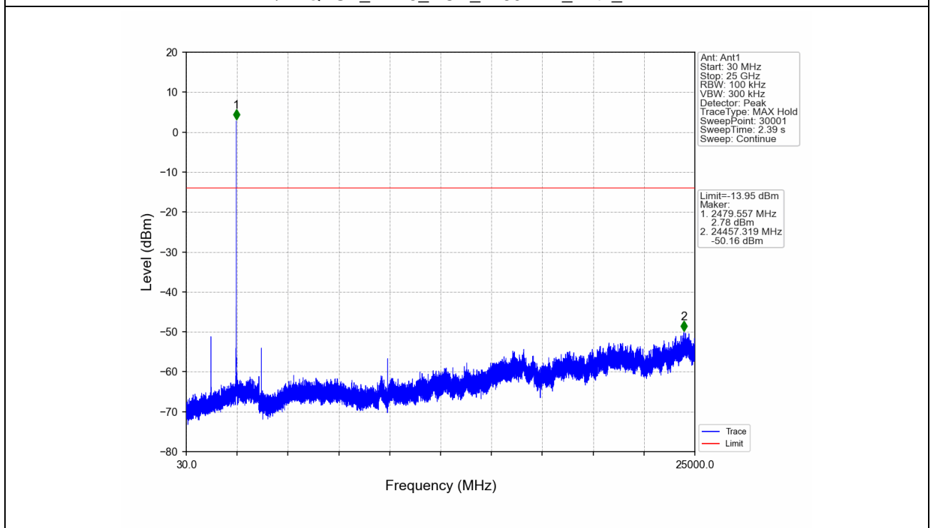
Pi/4DQPSK_2DH5_HCH_2480MHz_Ant1_NTNV
