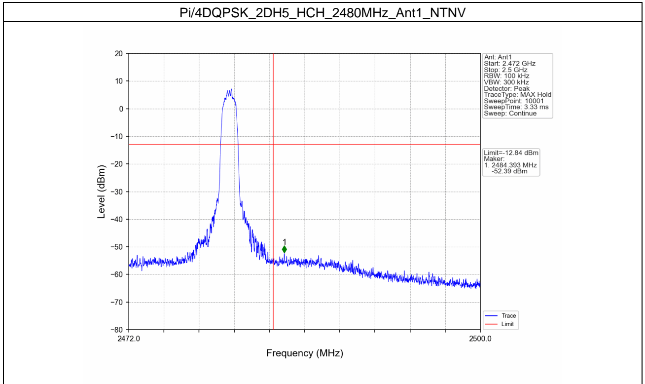
Pi/4DQPSK_2DH5_HCH_2480MHz_Ant1_NTNV
