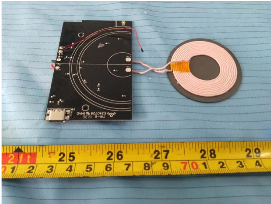
EUT – Main Board 1 Rear Cover off View
