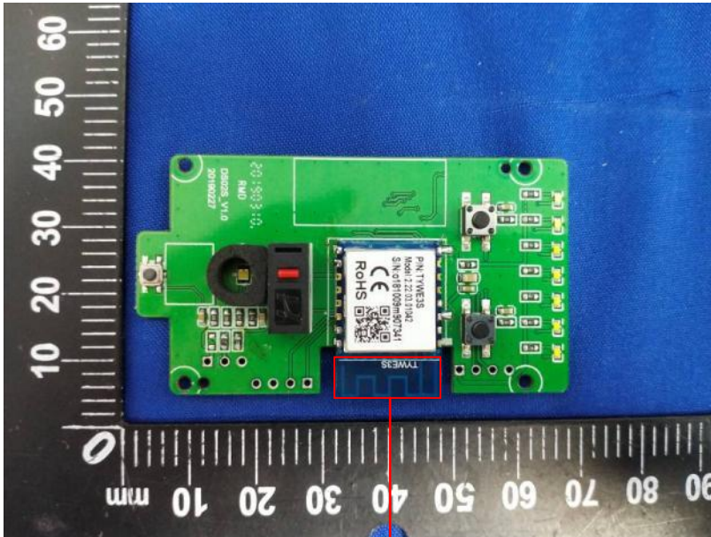
RF Antenna
