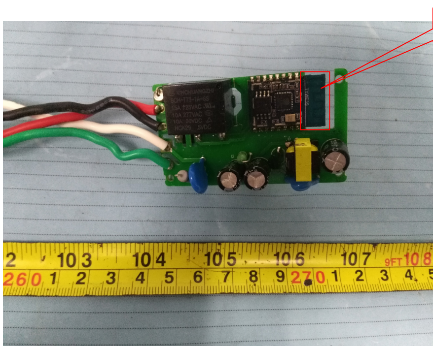
EUT – Main Board 2 Bottom Shielding off View
