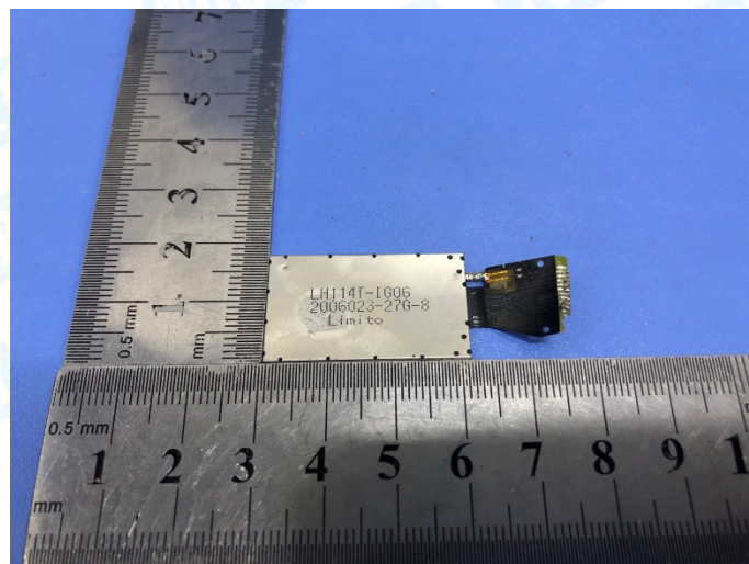
Photo 10 Appearance of PCB
