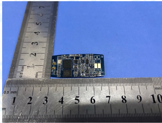
Photo 12 Appearance of PCB
