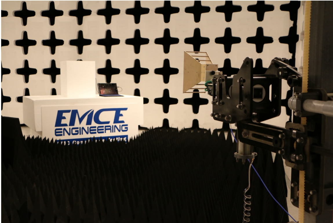
Radiated Emissions - Horn Antenna @ 3 Meters Measuring 1 GHz – 25 GHz
