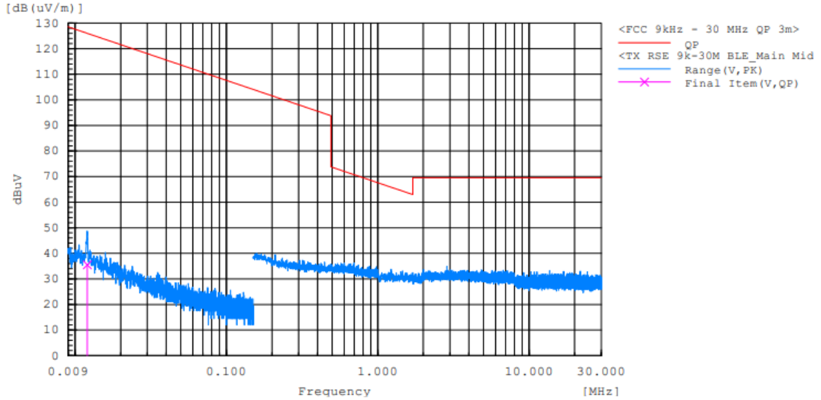
Radiated Spurious Emission 9 kHz – 30 MHz (Antenna Position 180°) : BLE MCU (CH 19 : 2440 MHz)
