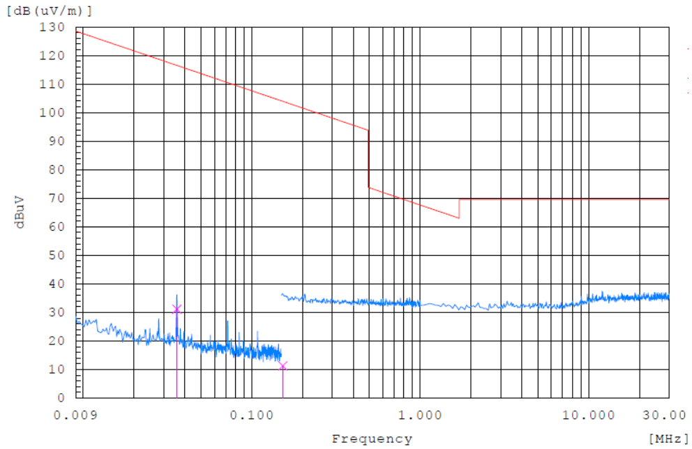
Radiated Spurious Emission 9 kHz – 30 MHz (Antenna Position 180°)
