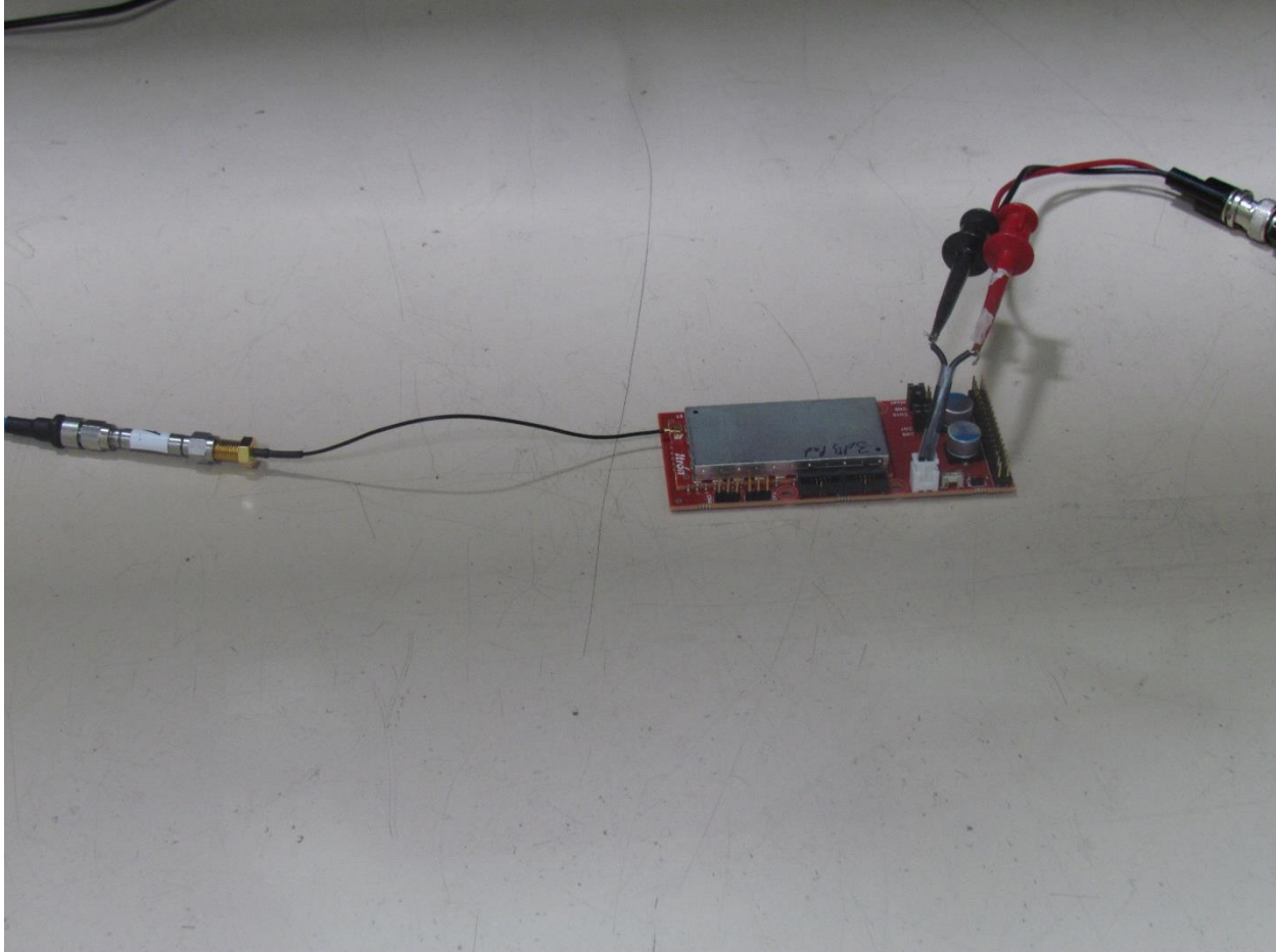
Conducted RF
