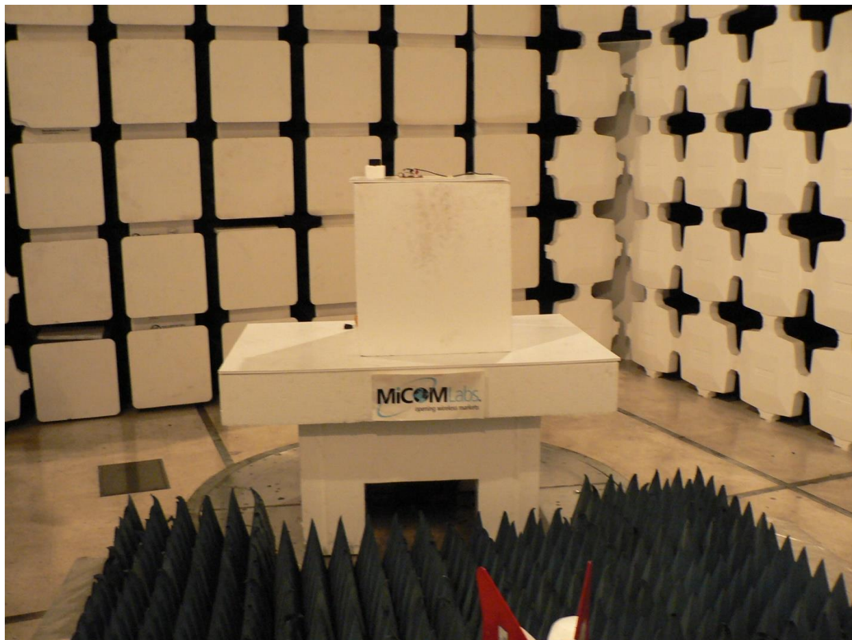
ITRO09 TX Spurious WPANT 1-10GHz
