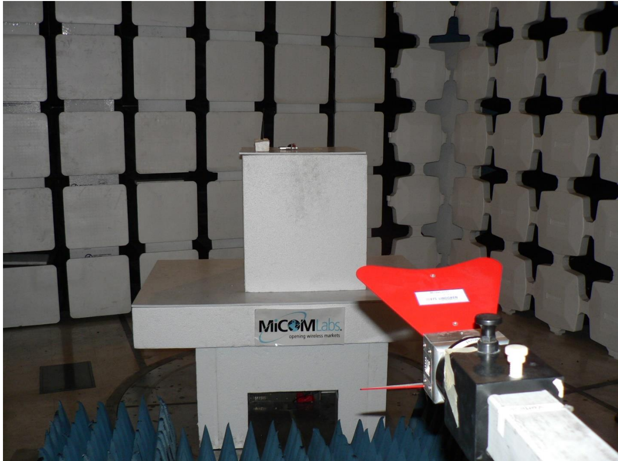
ITRO09 TX Spurious Laird 1-10GHz
