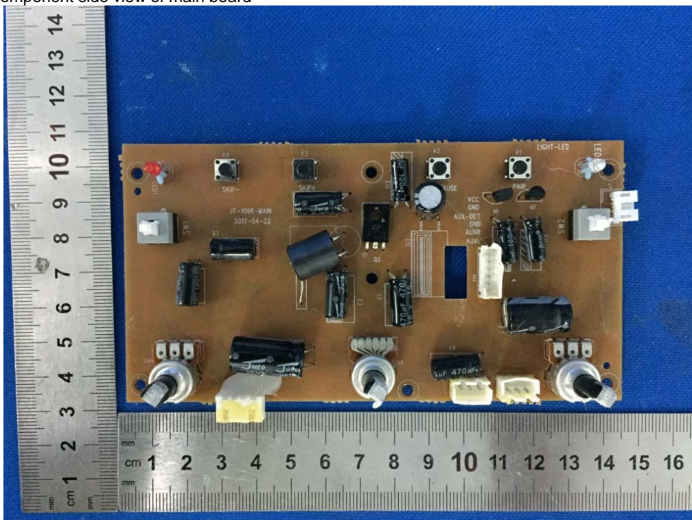
Fig. 16 Component side view of main board
