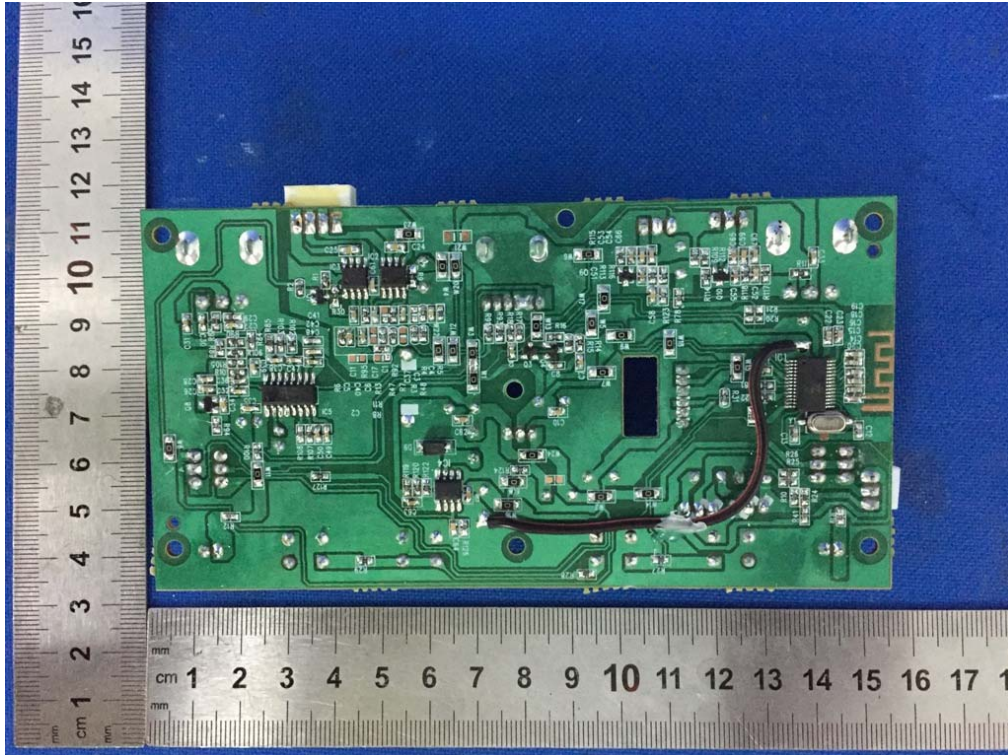
Fig. 15 Trace side view of main board
