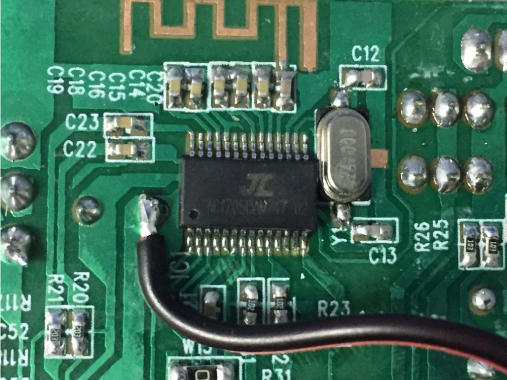
Fig. 17 BT Chip view
