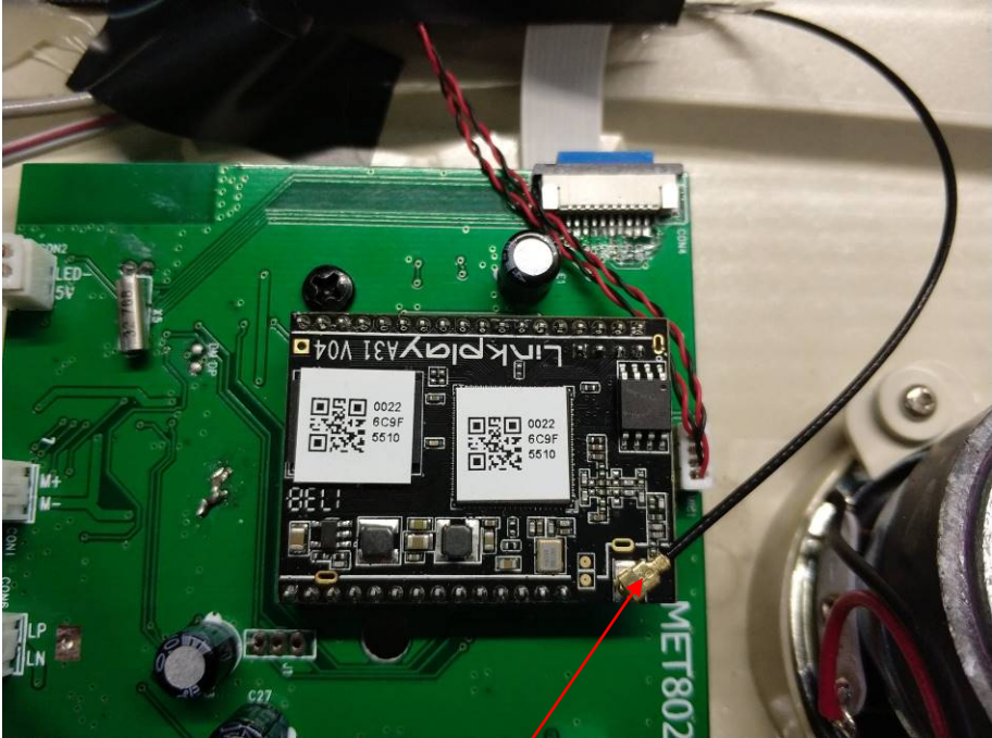
Wifi Antenna
