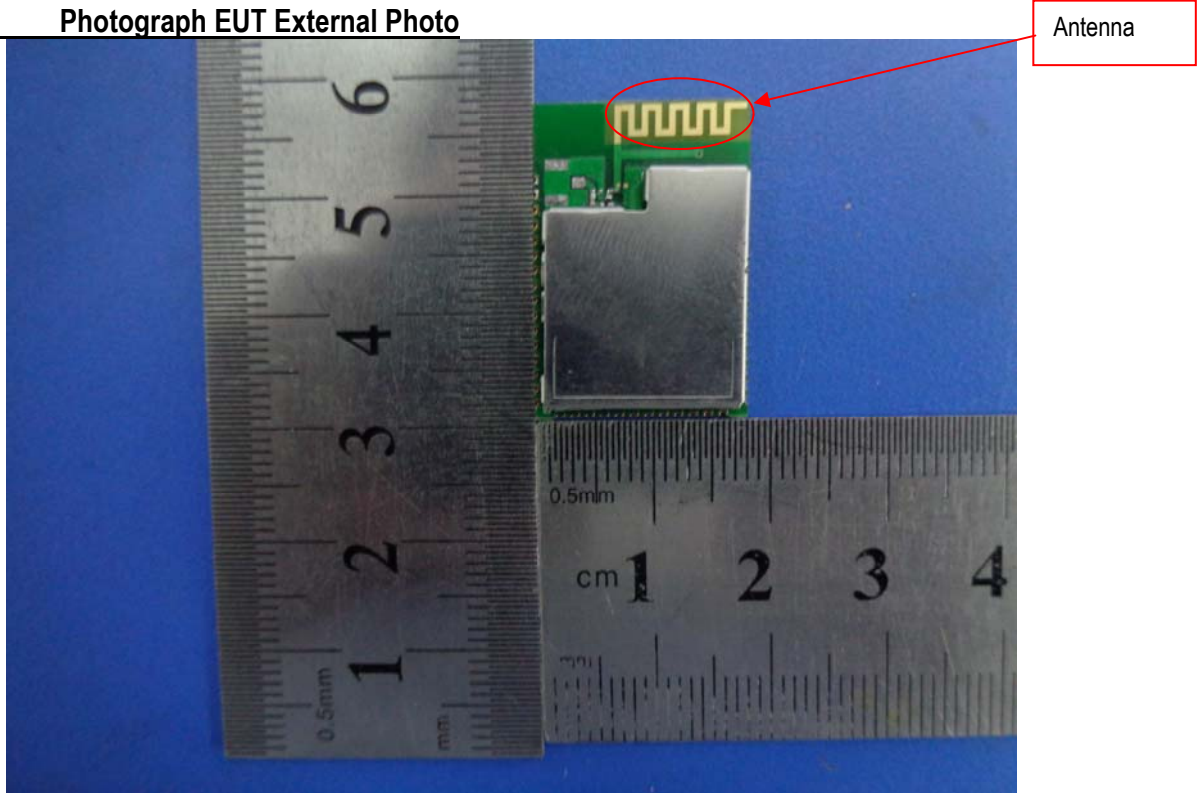
Front View of EUT
