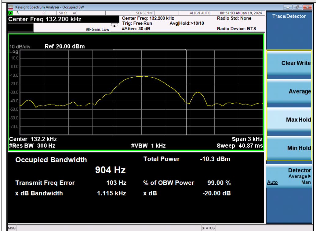
Test_Graph_ASK_Coil ANT_ 132.2kHz _ -20dB Bandwidth
