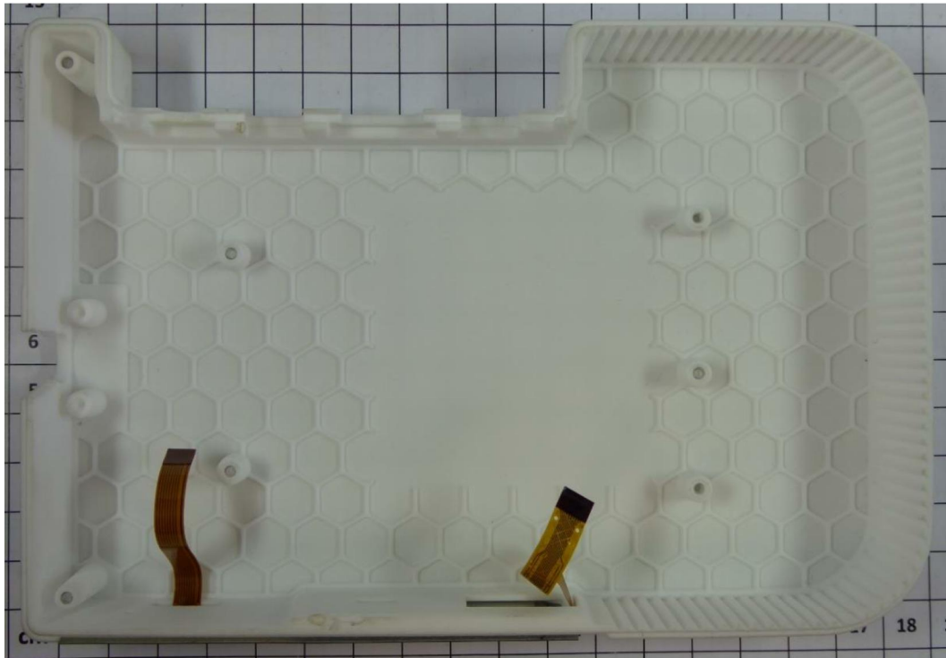
Enclosure bottom shell with touch keypad & display connecting cables:
