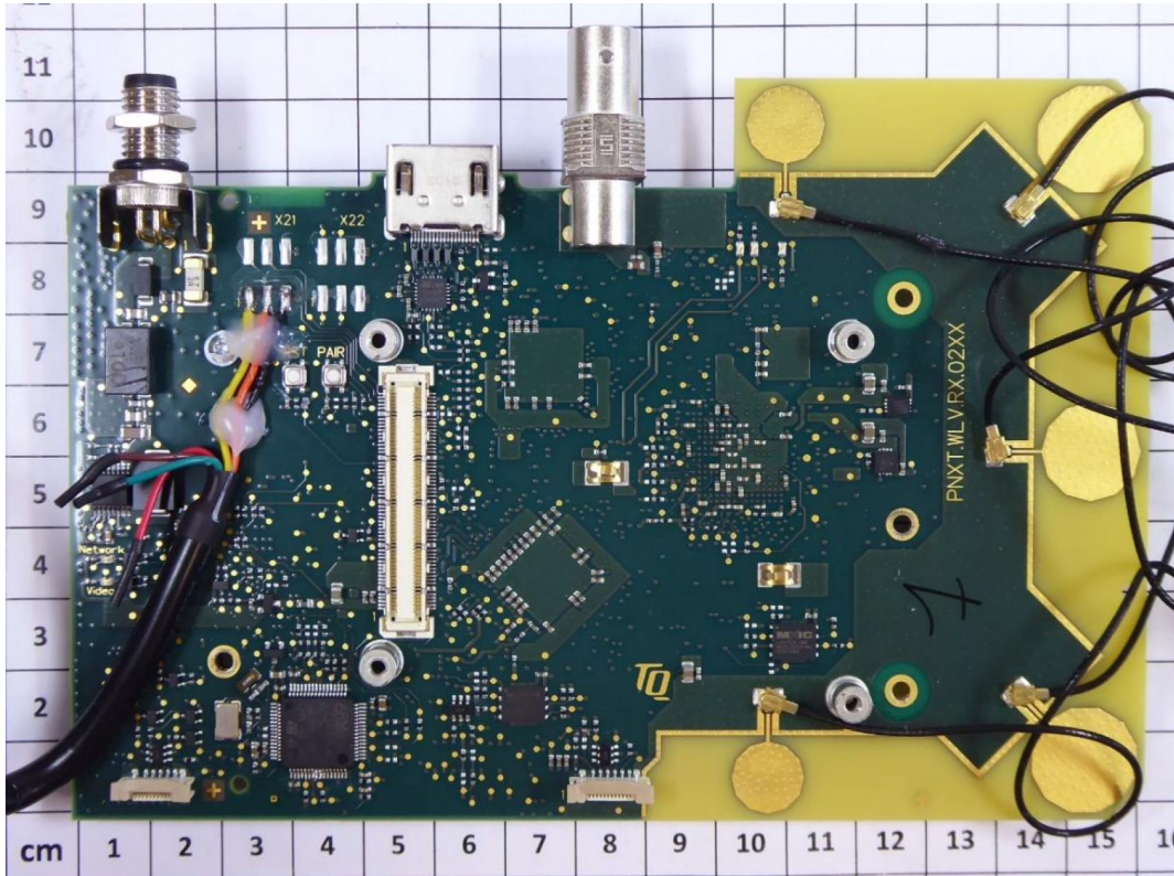
Amimon AMN42012 Draco Receiver - Various views:
