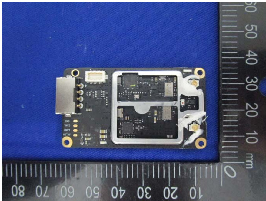
EUT –Wireless Module RF Board Top View
