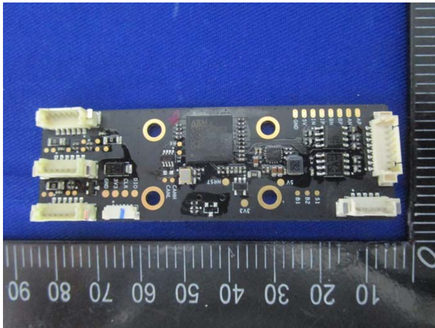
EUT –Wheel Controller Control Board Top View
