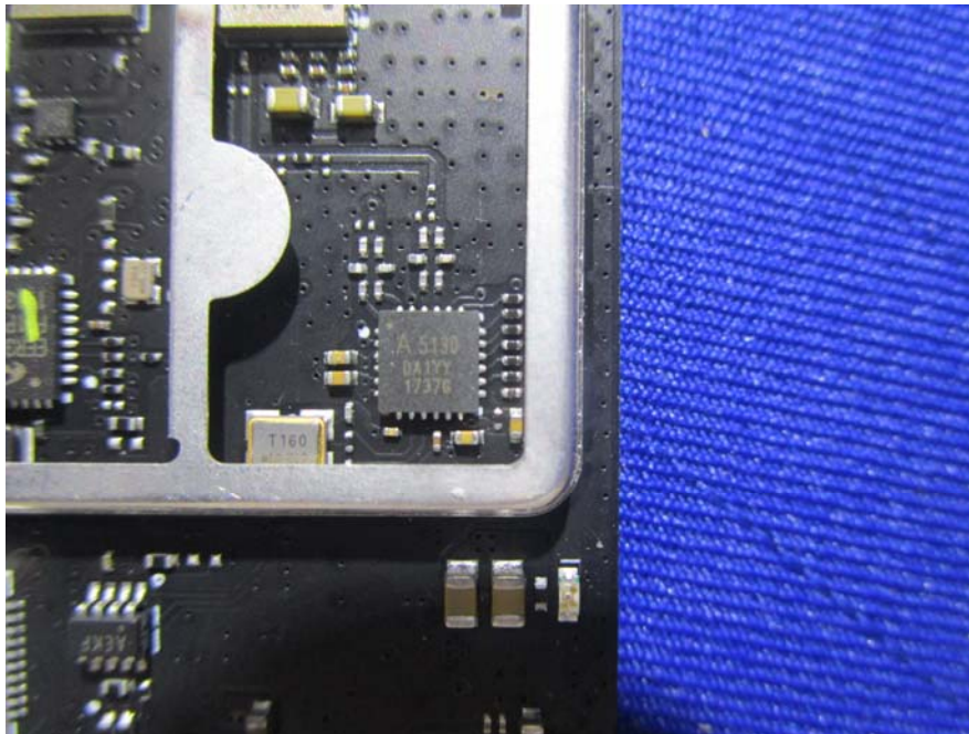
EUT –Wireless Module 5.8G Chip View
