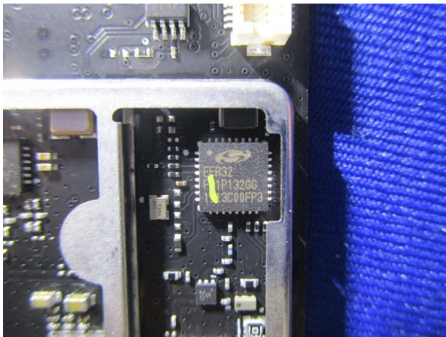
EUT –Wireless Module 2.4G Chip View
