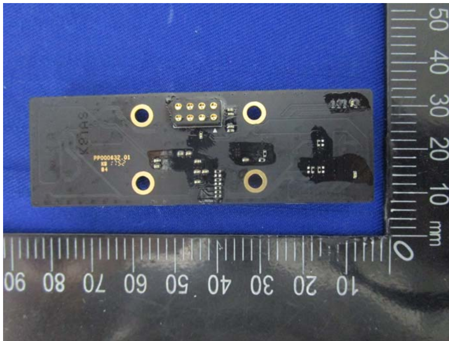
EUT –Wheel Controller Control Board Bottom View
