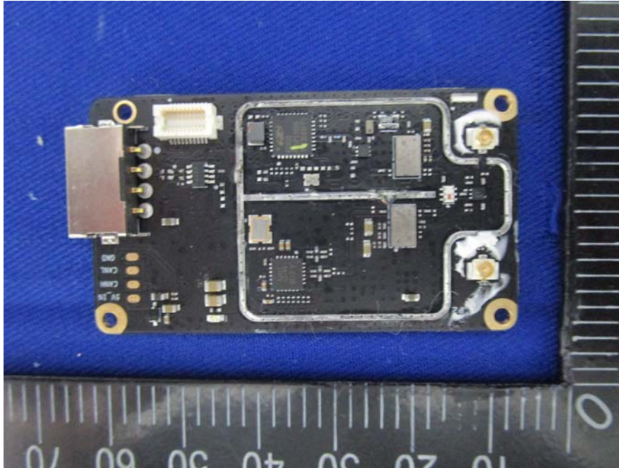
EUT –Wireless Module RF Board Top Uncover View
