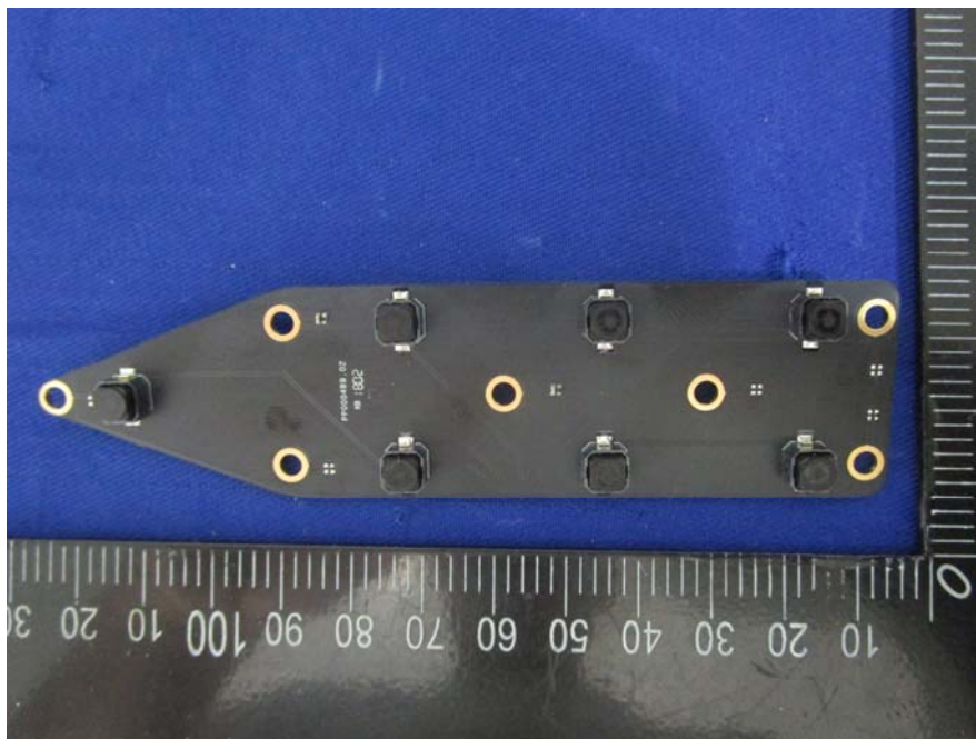
EUT – Button Control Board Top View
