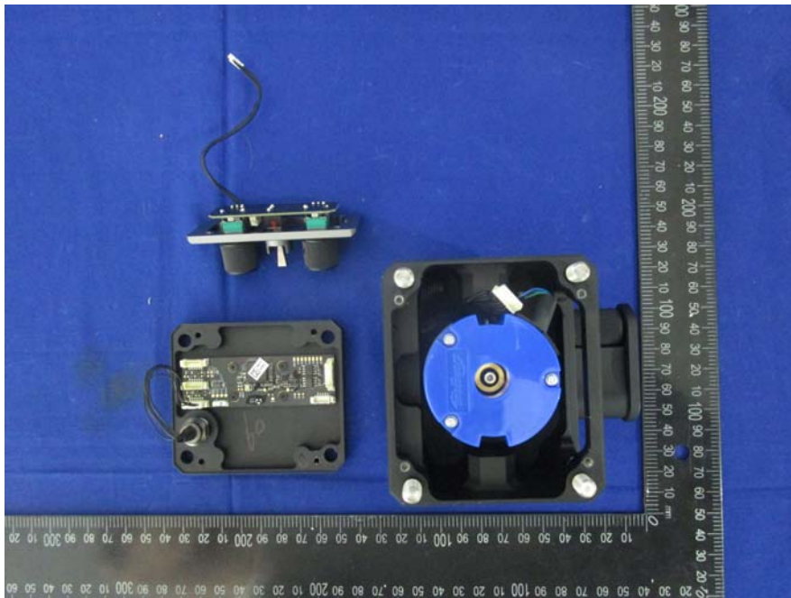
EUT –Wheel Controller Uncover View
