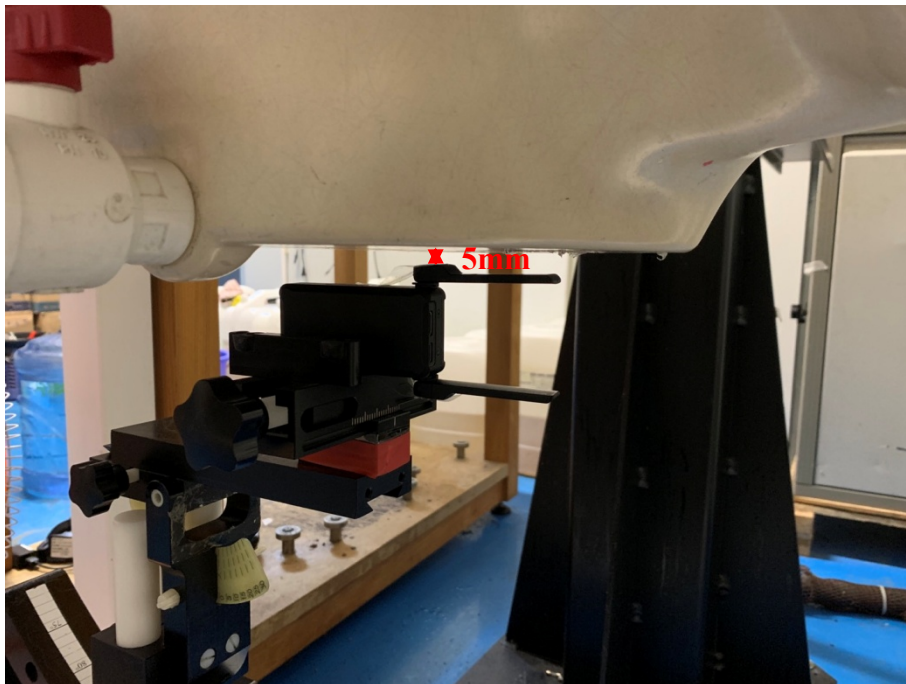
Front Side With Antenna Unfold (Chain 1)Setup Photo(5mm)
