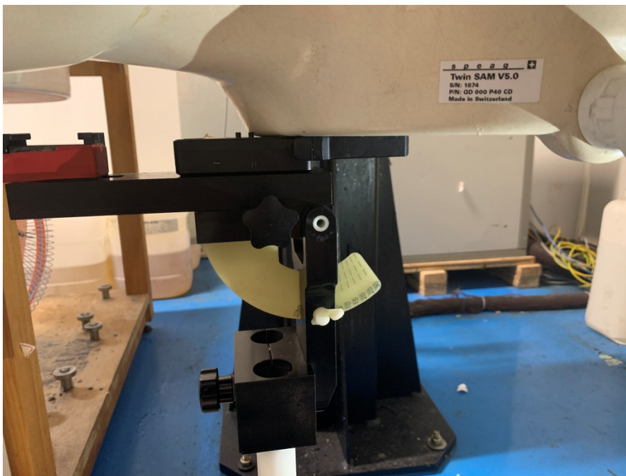
Extremity(Hand) Bottom With Antenna Unfold Setup Photo(0mm)
