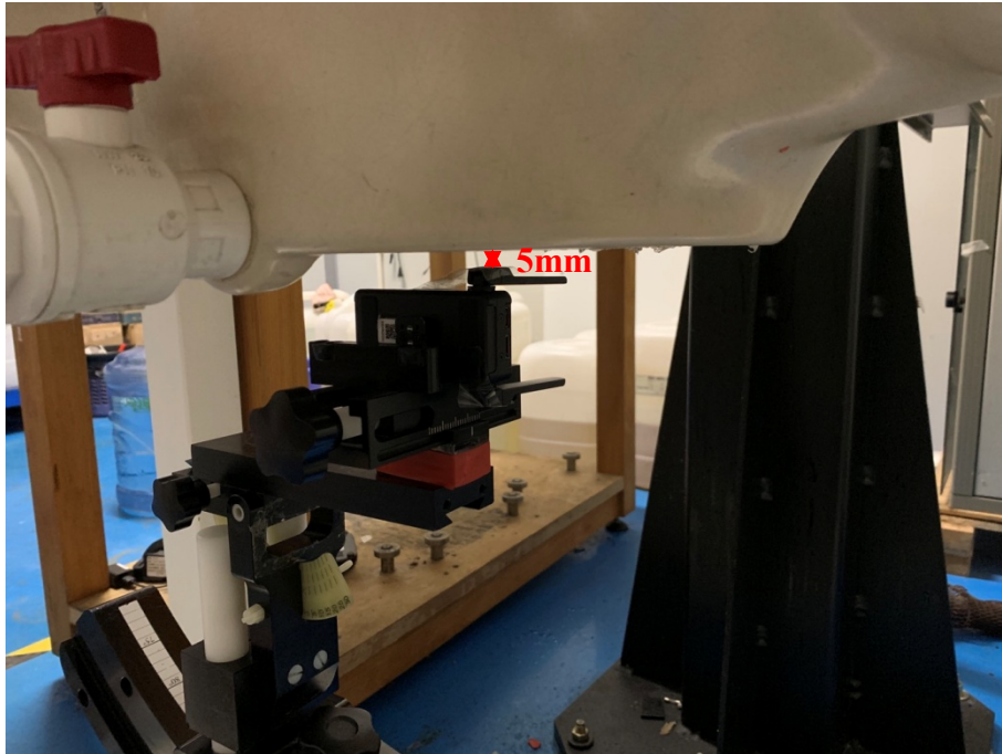
Back Side With Antenna Fold(Chain 0) Setup Photo(5mm)
