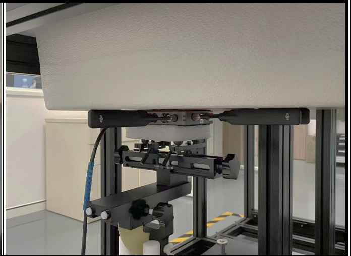
Front Face of EUT with 0 cm Gap_ Antenna Vertical
