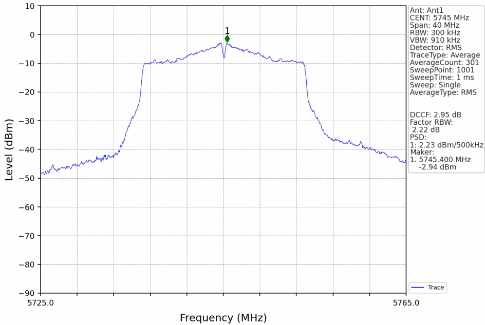
802.11ac(VHT20)_LCH_5745MHz_MIMO_NTNV
