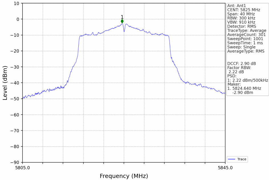
802.11ac(VHT20)_HCH_5825MHz_MIMO_NTNV
