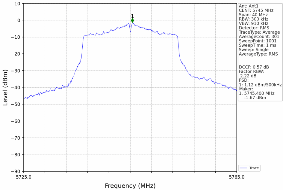
802.11ax(HEW20)_LCH_5745MHz_RU242_Left_MIMO_NTNV
