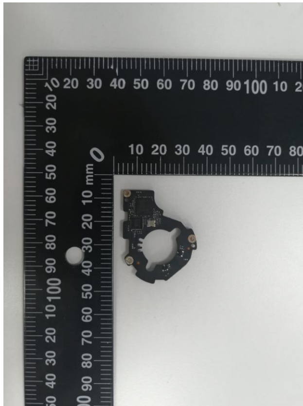
Photo-Internal view 10
