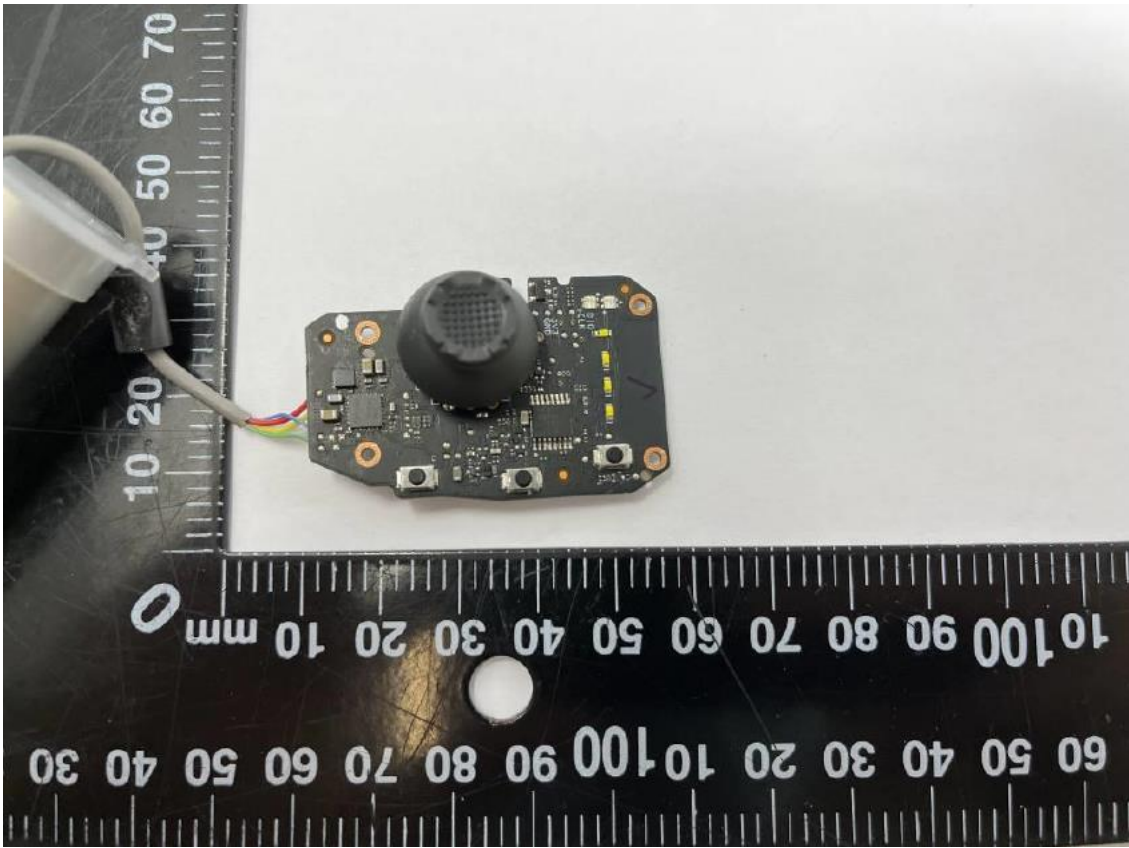
Photo-Internal view 6
