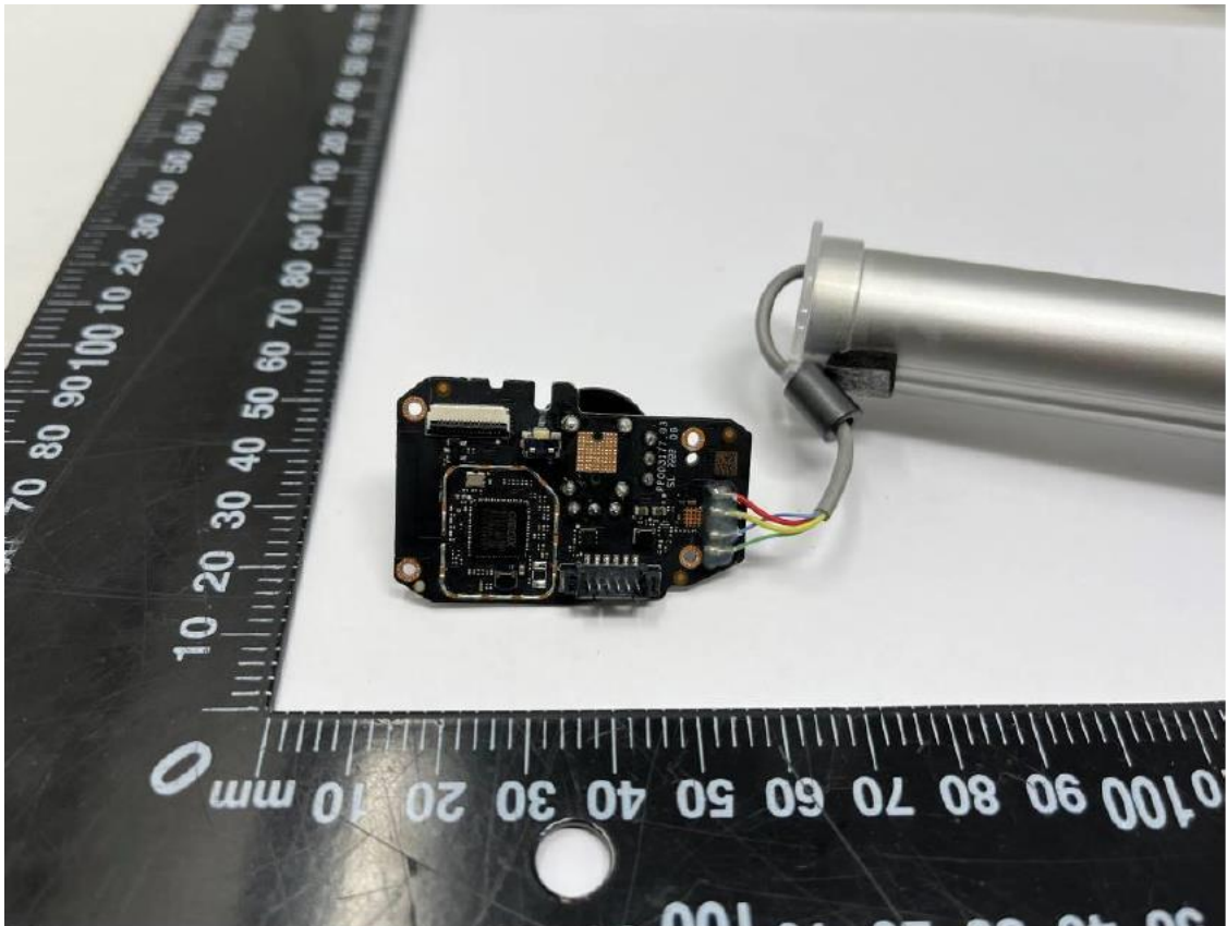
Photo-Internal view 4
