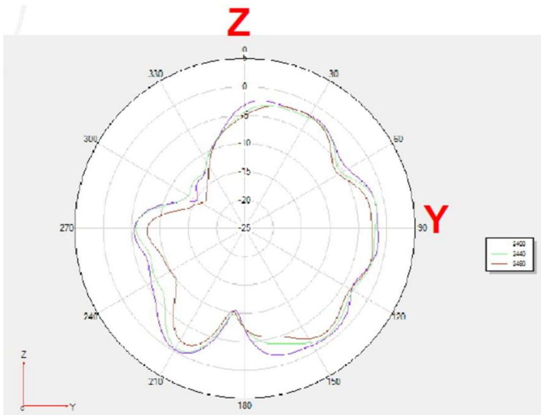
GFSK Antenna
