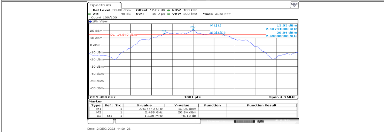
SRD-2M_Ant1_2438
