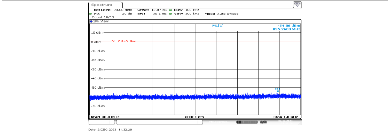
SRD-2M_Ant1_2438_0~Reference
