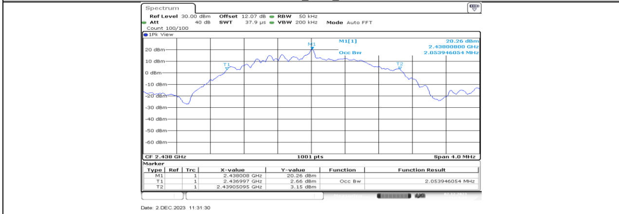
SRD-2M_Ant1_2438
