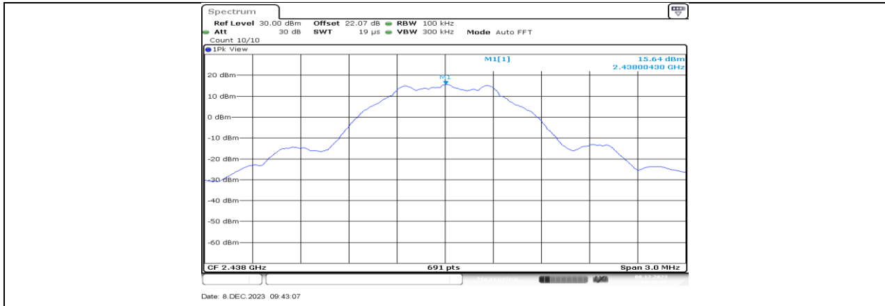
SRD-1M_Ant1_2438_0~Reference
