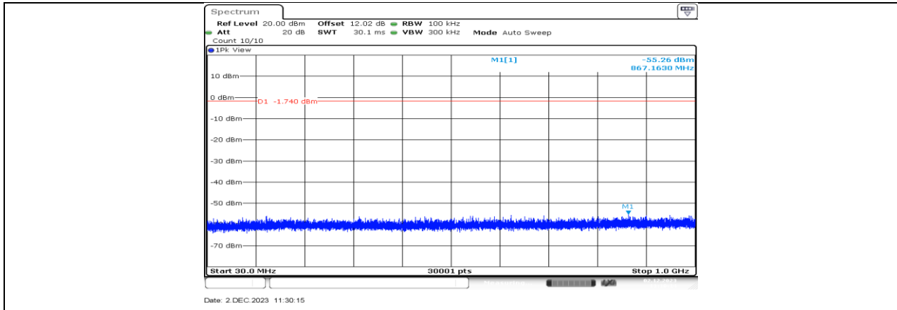
SRD-2M_Ant1_2402_30~1000
