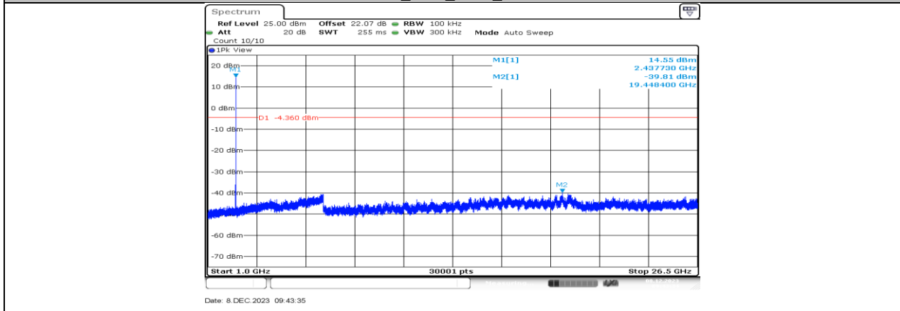
SRD-1M_Ant1_2438_1000~26500
