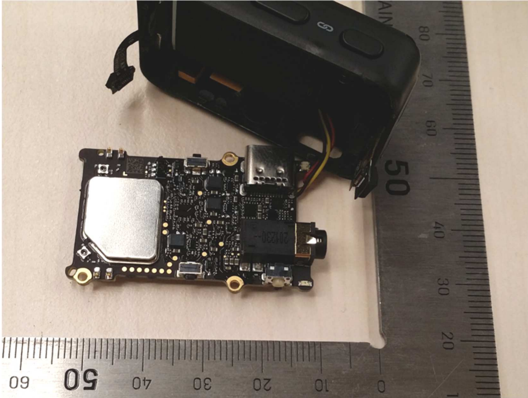
Figure 3: Internal view -3
