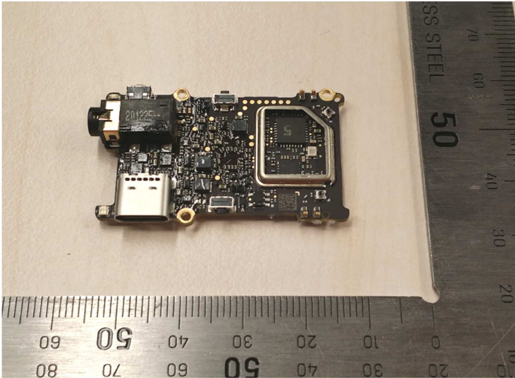
Figure 6: Mainboard view -2
