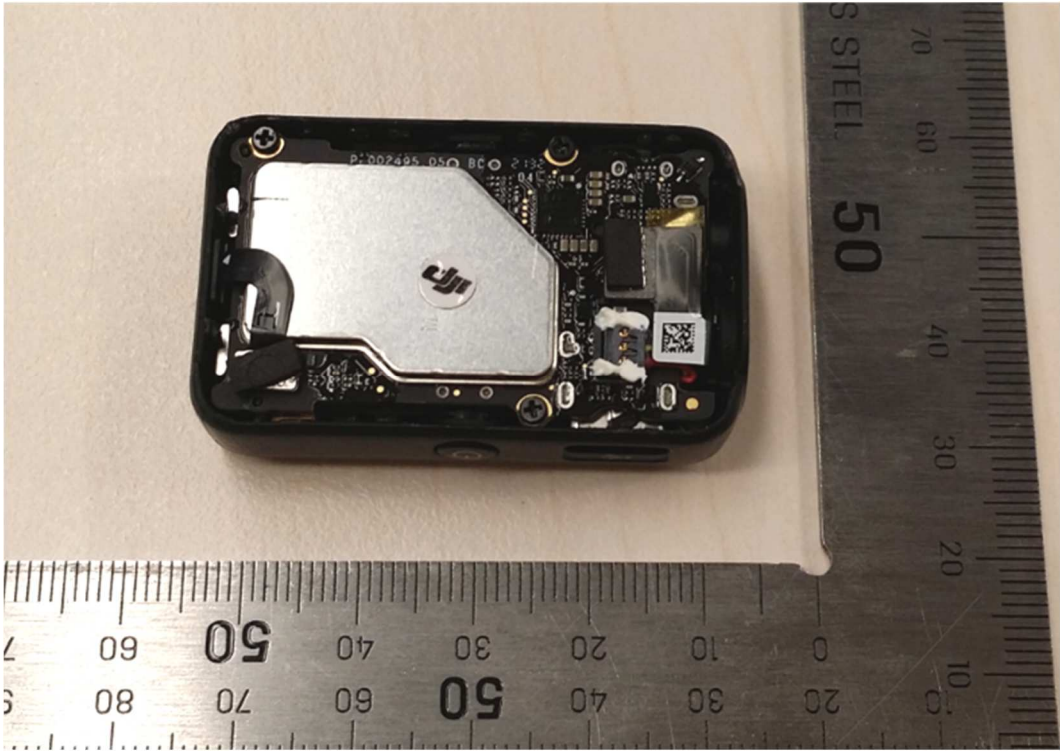
Figure 1: Internal view -1
