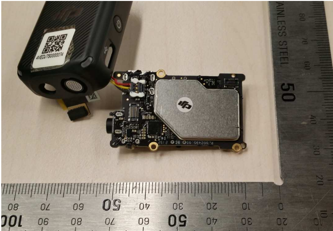
Figure 2: Internal view -2
