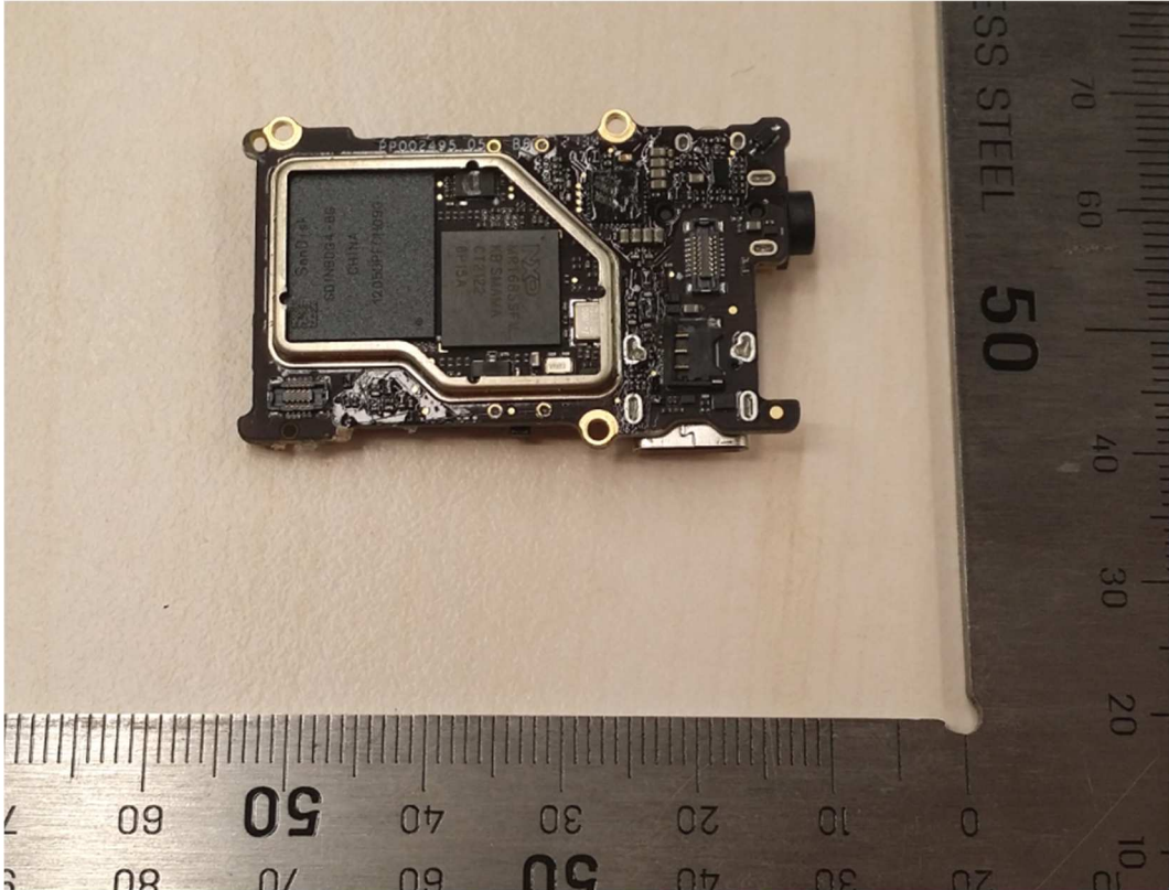
Figure 5: Mainboard view -1
