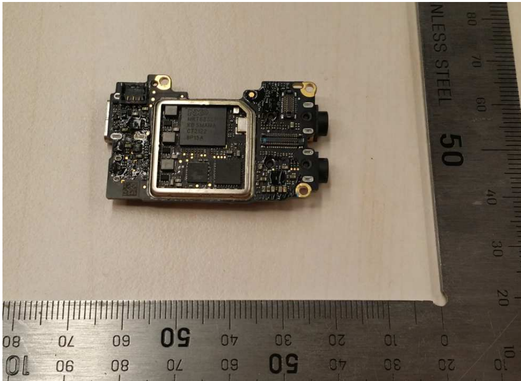
Figure 5: Mainboard view -2
