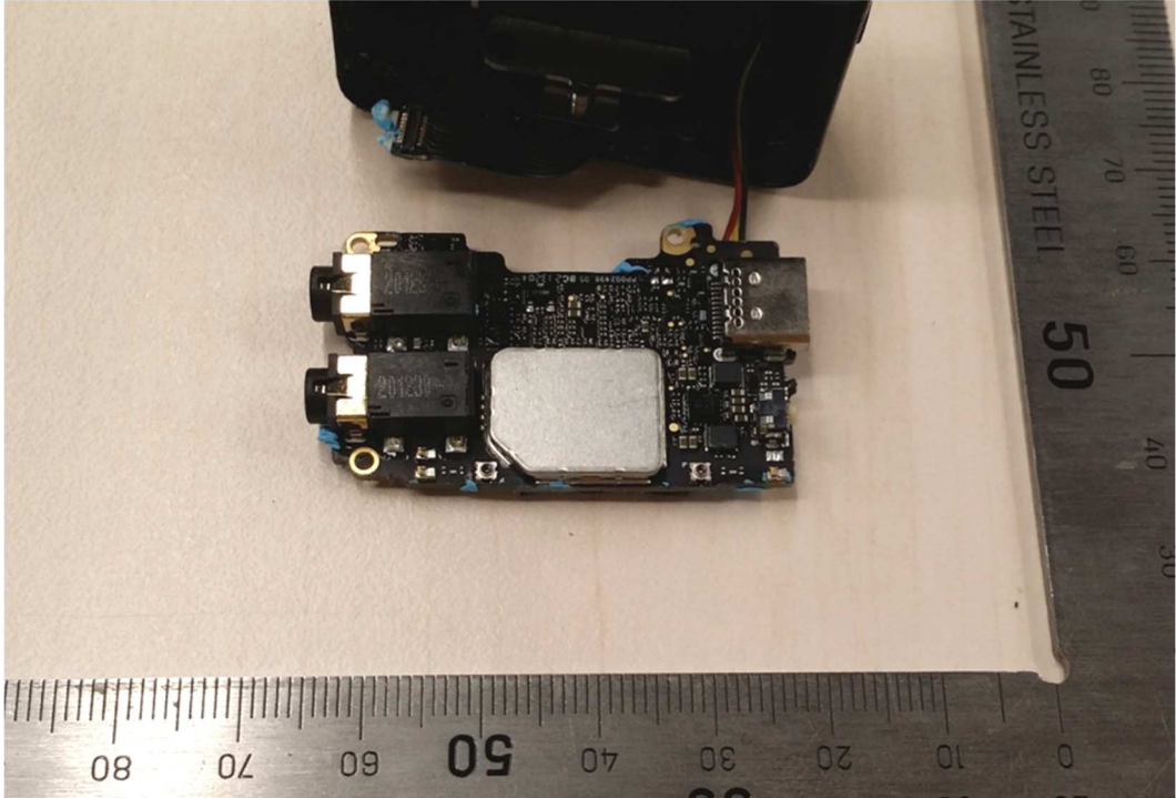
Figure 2: Internal view -2
