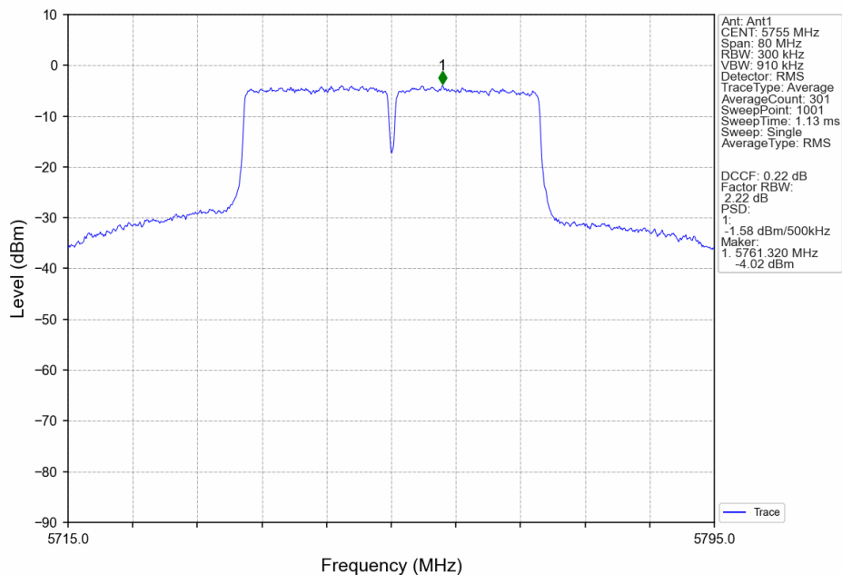
802.11ax(HEW40)_LCH_5755MHz_SU_Ant1_NTNV
