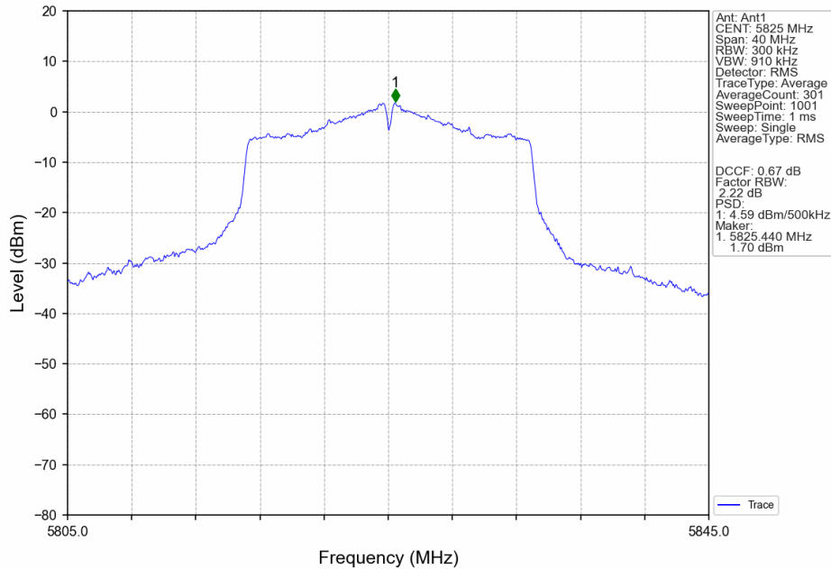
802.11ac(VHT20)_HCH_5825MHz_MIMO_NTNV
