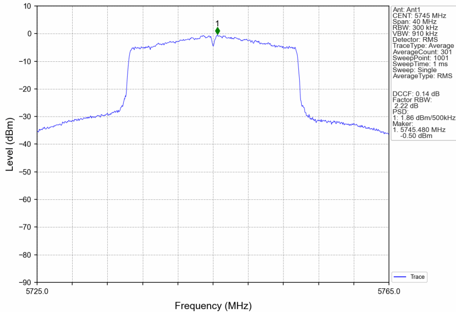
802.11ax(HEW20)_LCH_5745MHz_SU_MIMO_NTNV
