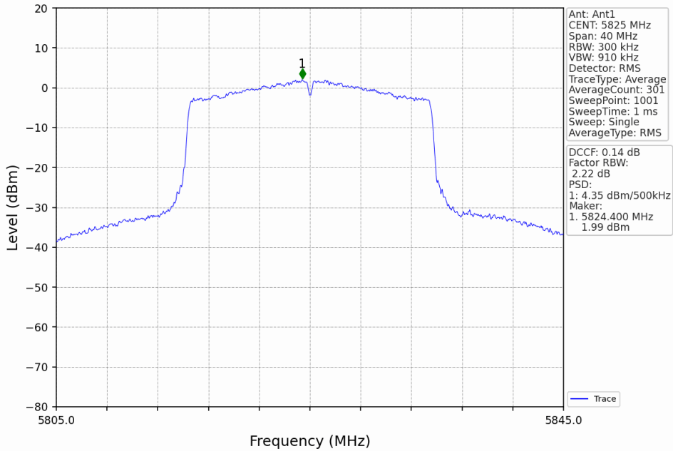
802.11ax(HEW20)_HCH_5825MHz_RU242_Left_MIMO_NTNV
