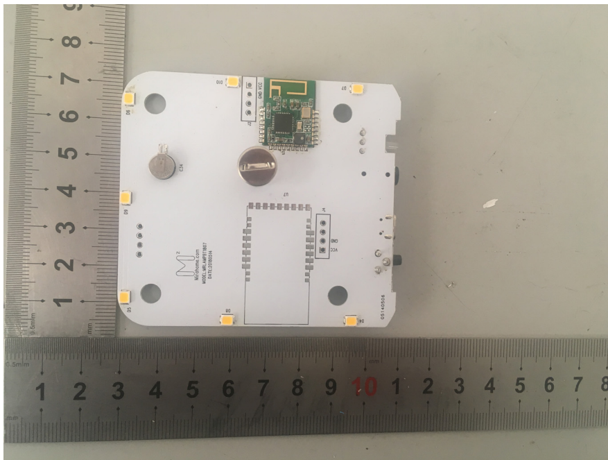
EUT – Antenna and Module View
