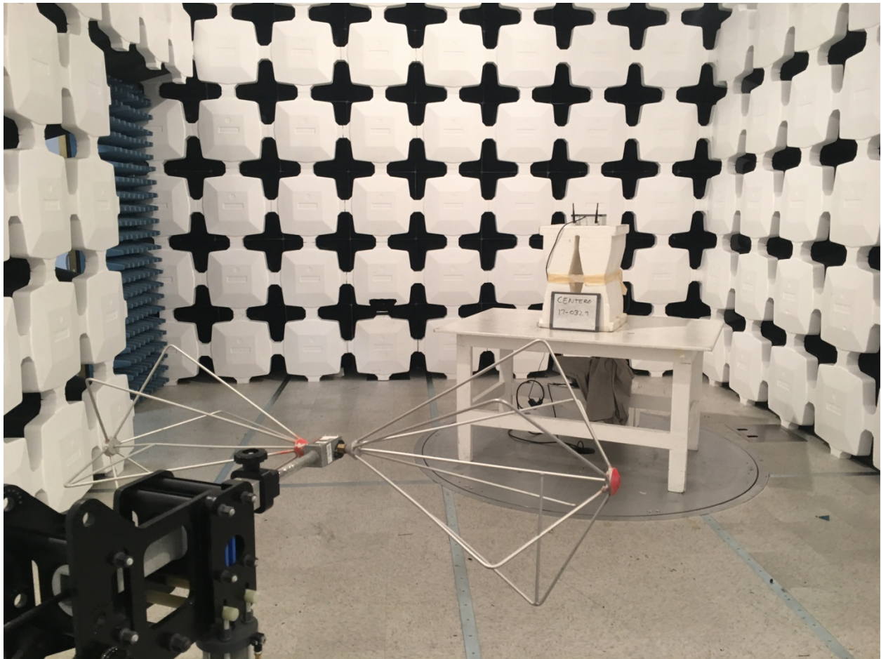
Figure 6. Radiated Emissions, 30-200 MHz
