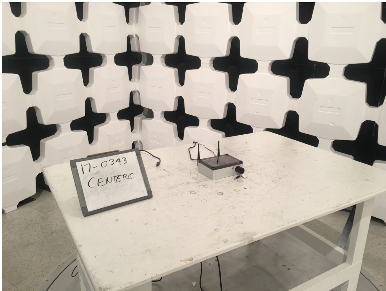
Figure 1. EUT Radiated Emissions Test Config Photo 1
