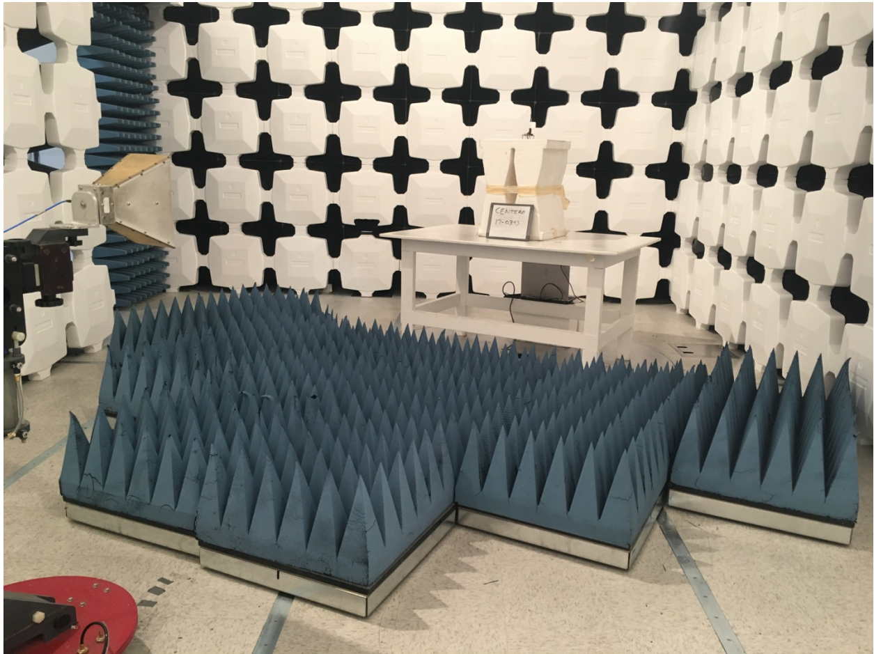
Figure 8. Radiated Emissions, Above 1 GHz
