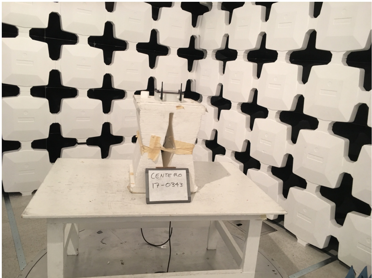
Figure 2. EUT Radiated Emissions Test Config Photo 2
