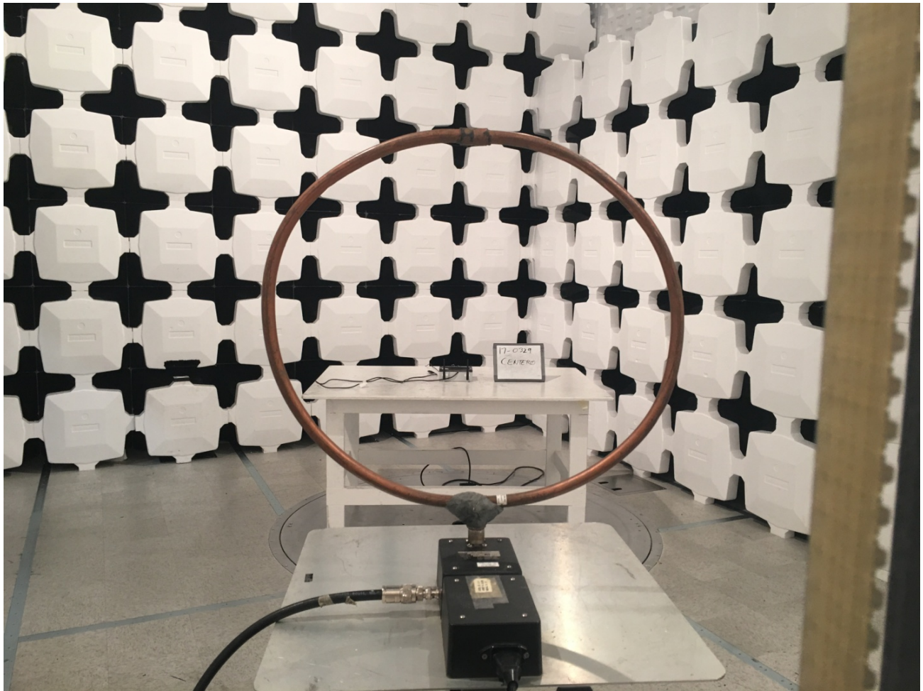
Figure 3. Spurious Radiated Emissions Below 30 MHz, X Polarity
