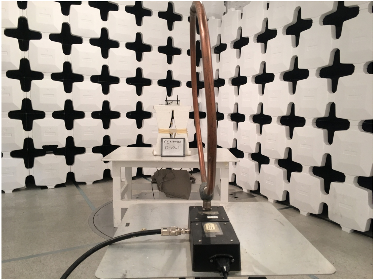
Figure 4. Radiated Emissions Below 30 MHz, Y-Polarity
