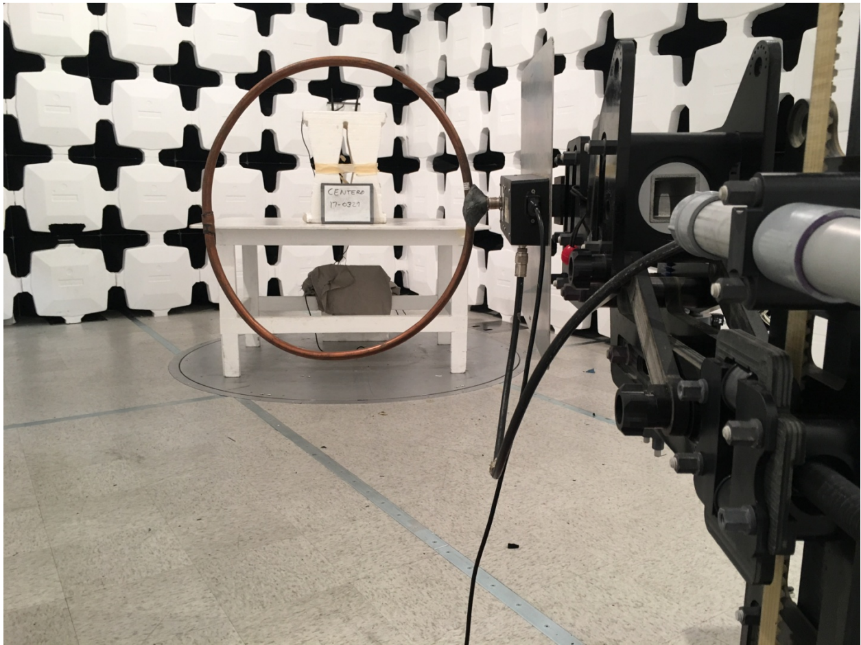
Figure 5. Radiated Emissions Below 30 MHz, Z-Polarity
