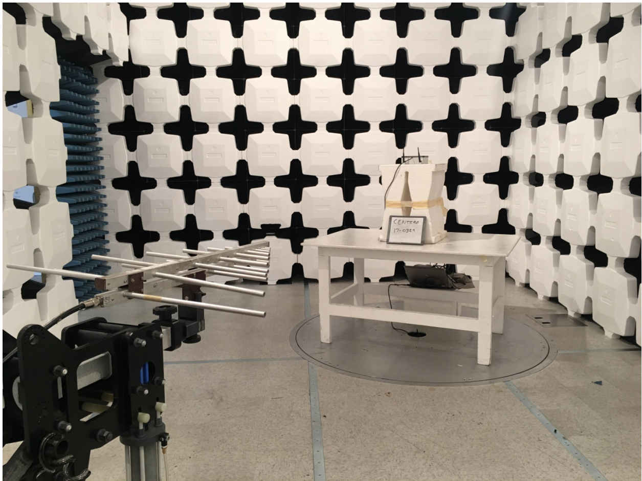
Figure 7. Radiated Emissions, 200-1000 MHz
