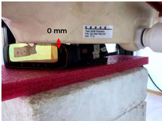
Fig.5 EUT 4 to flat phantom
