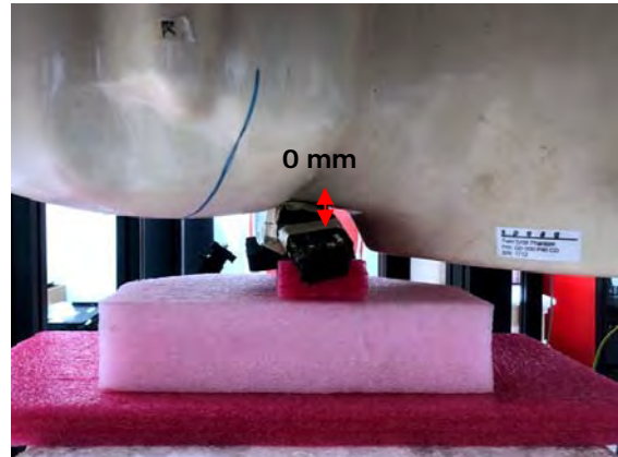
Fig.10 EUT 7 to flat phantom
