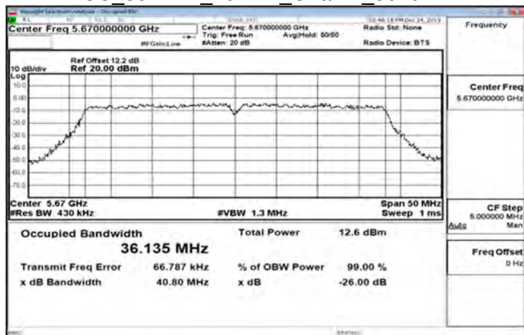
FCC 802.11n 40MHz_Chain1_5670MHz
