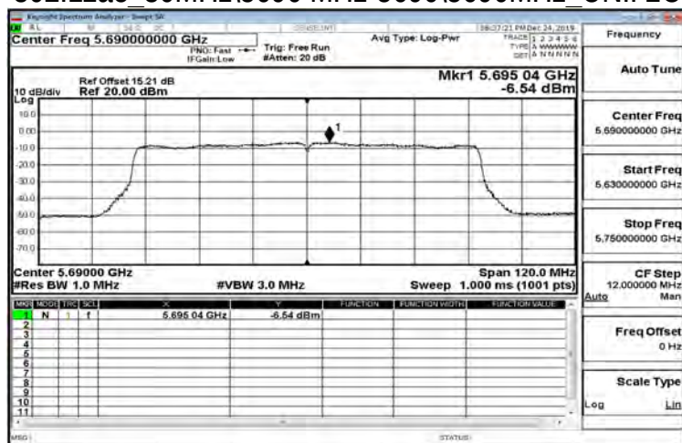
802.11ac 80MHz\5690 MHz-5690\5690MHz UNII 3
