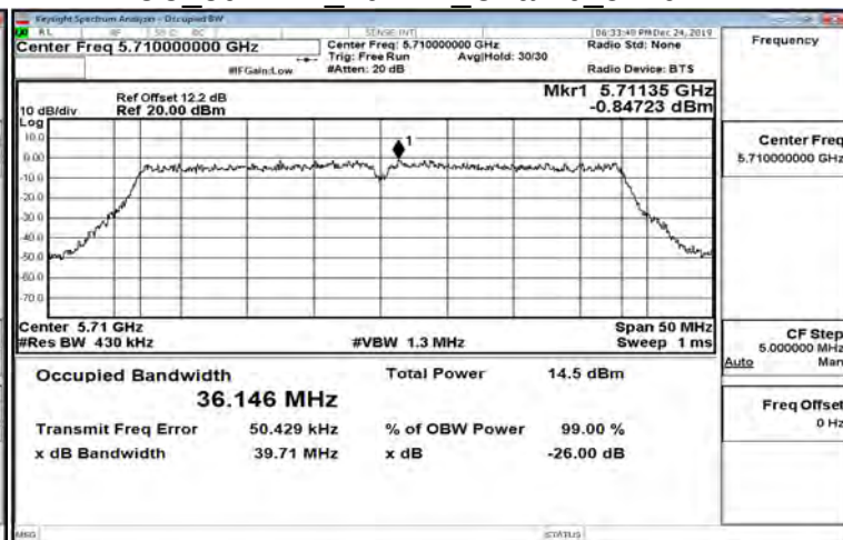
FCC 802.11n 40MHz_Chain0_5710MHz
