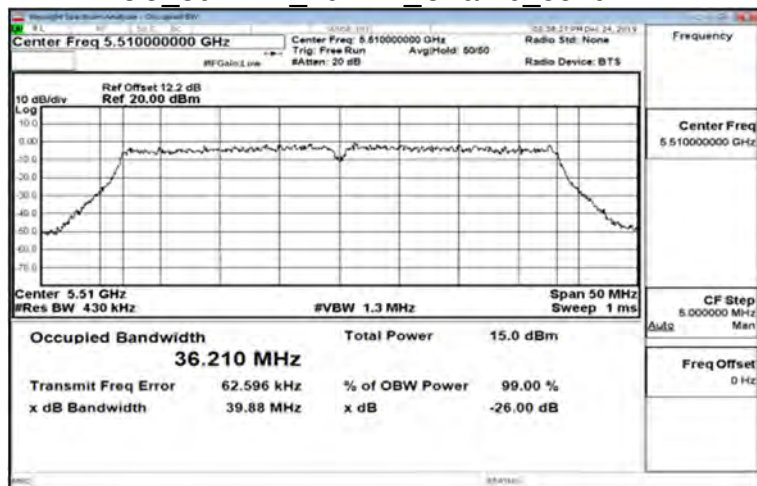
FCC 802.11n 40MHz_Chain0_5510MHz
