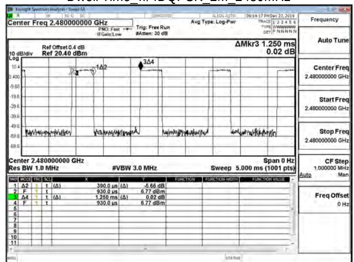
Dwell Time_π/4DQPSK_2M_2480MHz
