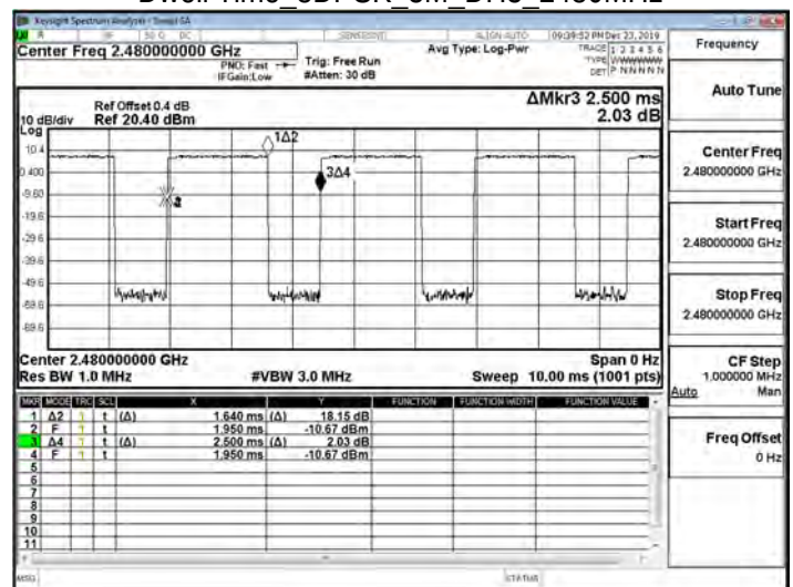
Dwell Time 8DPSK 3M_DH3_2480MHz
