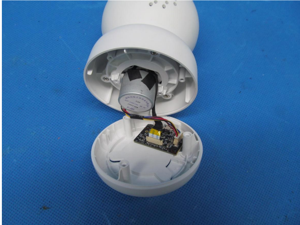
Photo 8. Internal view
