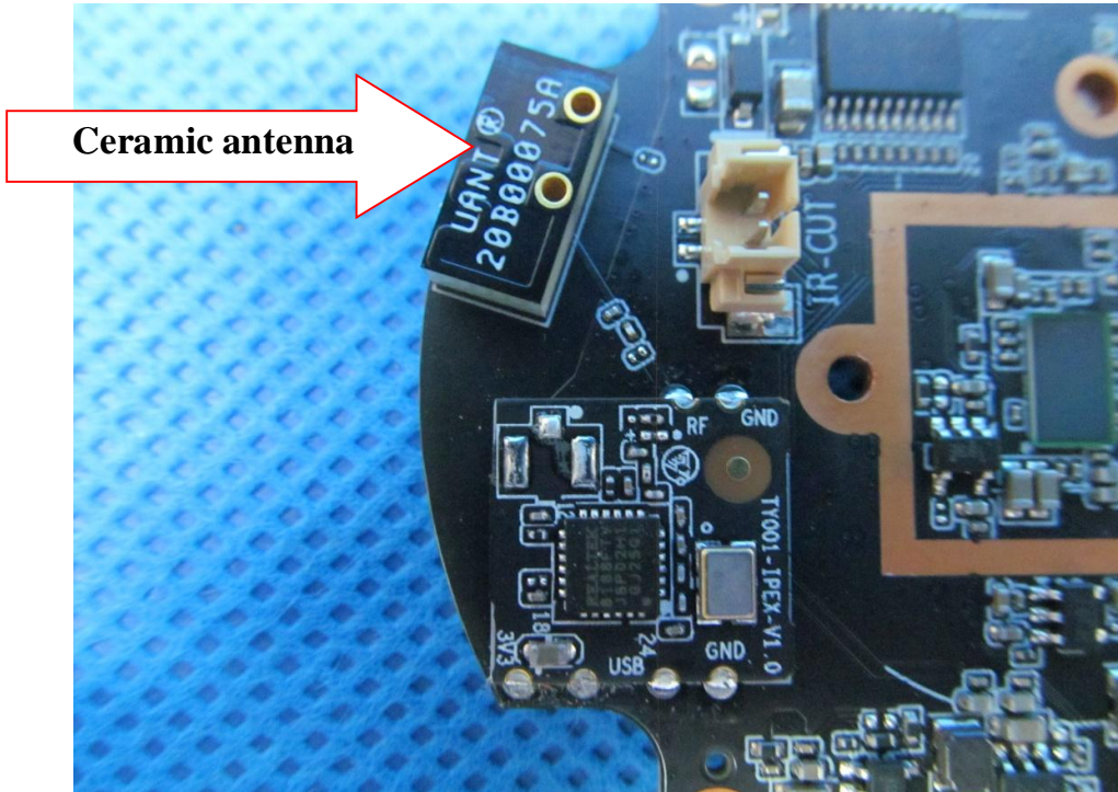
Photo 2. PCB view
