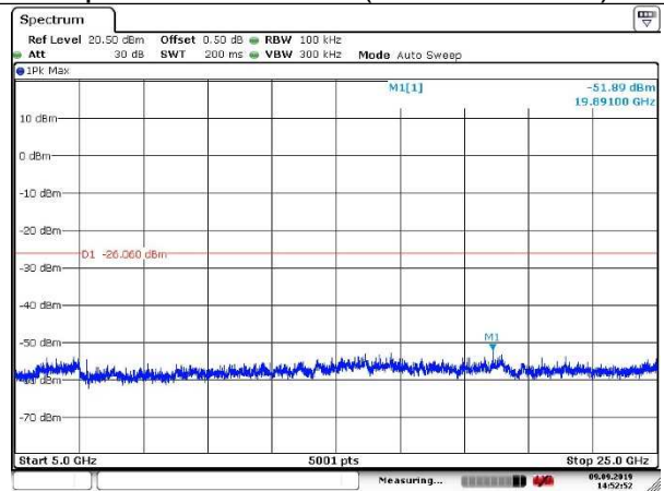
Spurious Emission (5GHz –25GHz)
