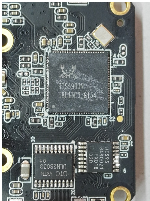
EUT-PCB-2 Bottom View
