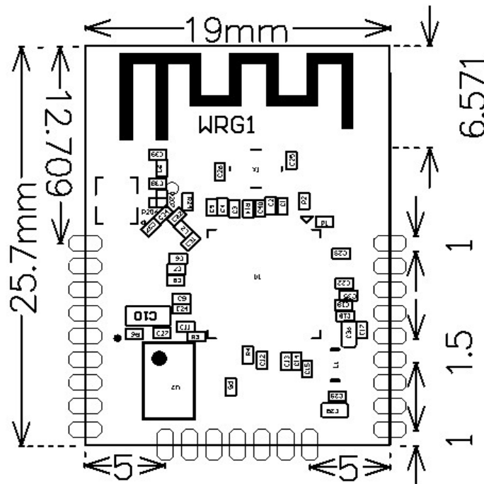
Figure 6.1 Module elevation
