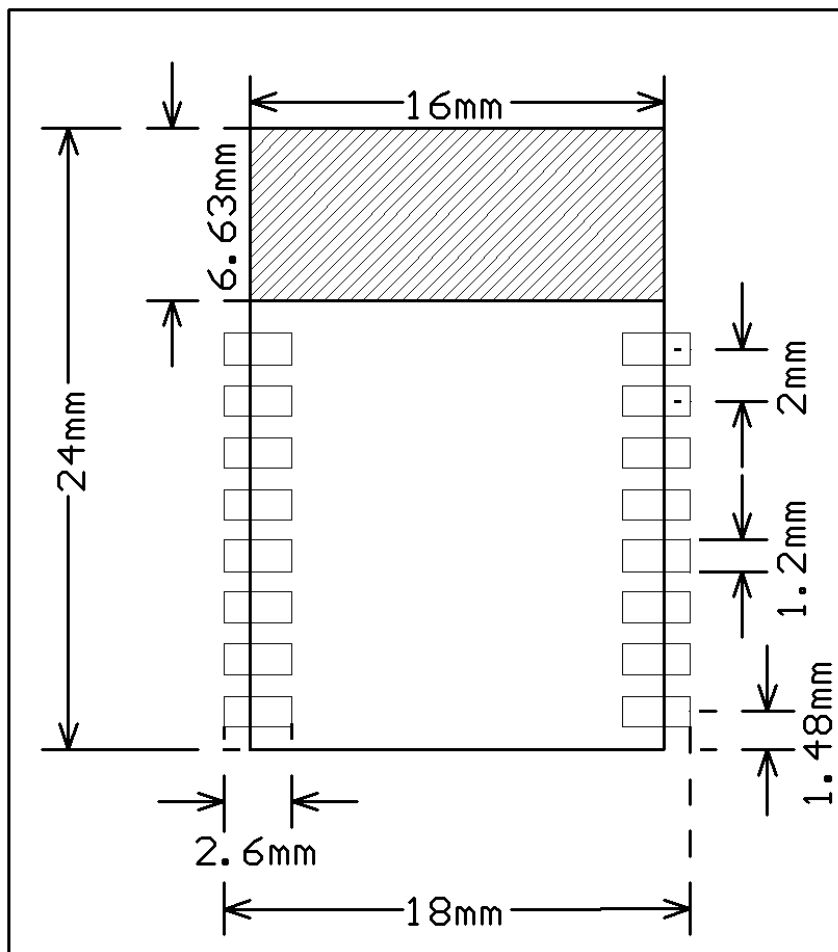
Figure 6.3. PCB footprint
