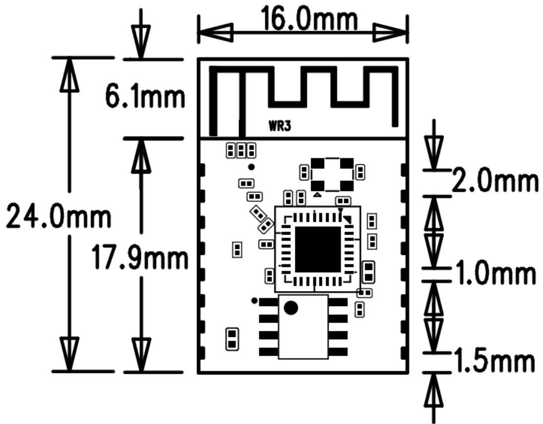
Figure 6.1. Top view of the module
