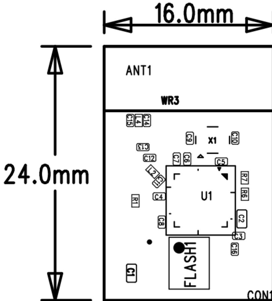
Figure 2.1. The dimensions of WR3
