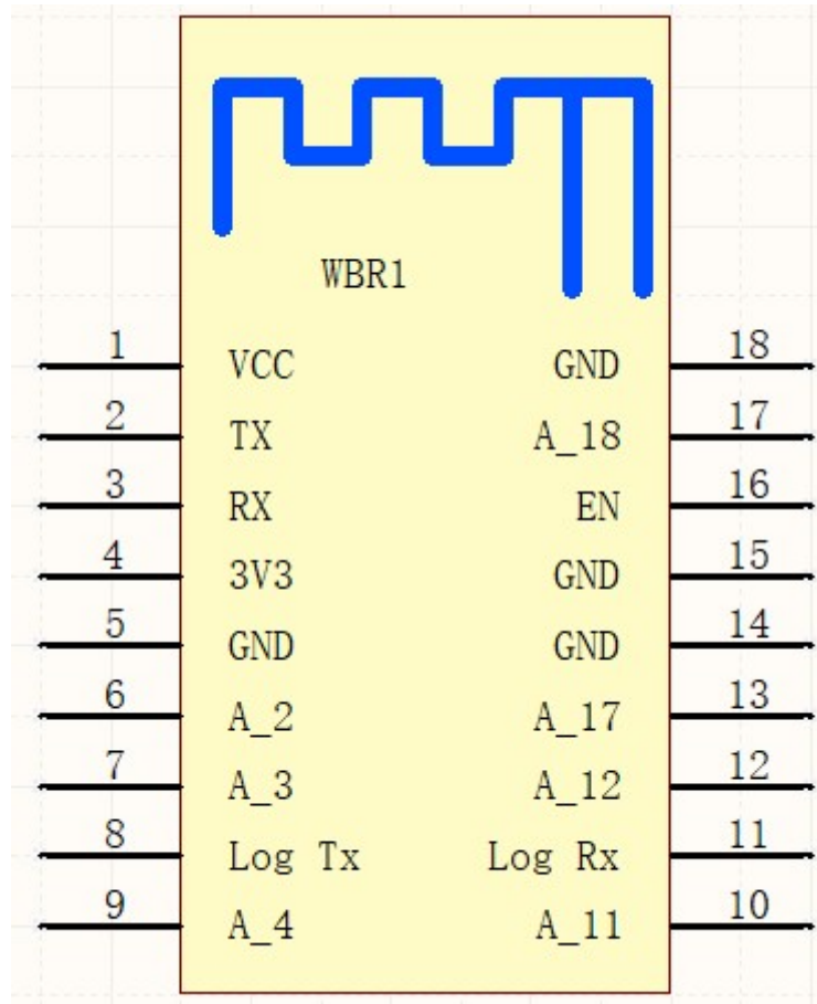
Figure 6-3 WBR1-IPEX pins
