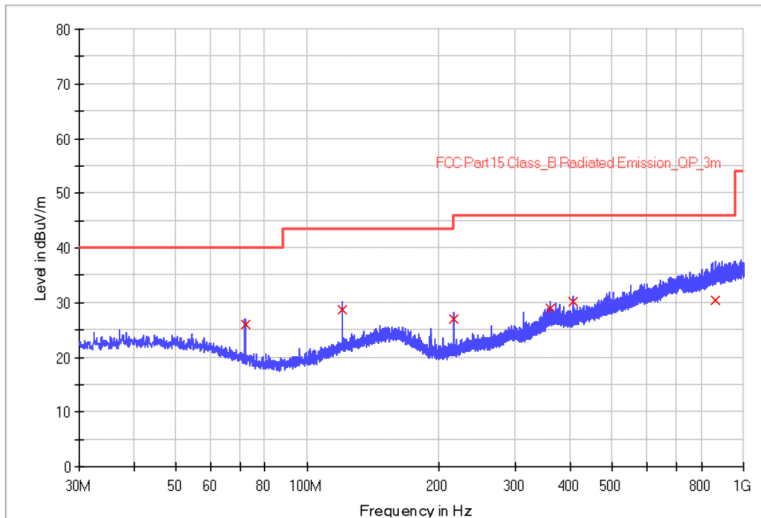
PE_VULB9168_pre_Cant_30-1000
