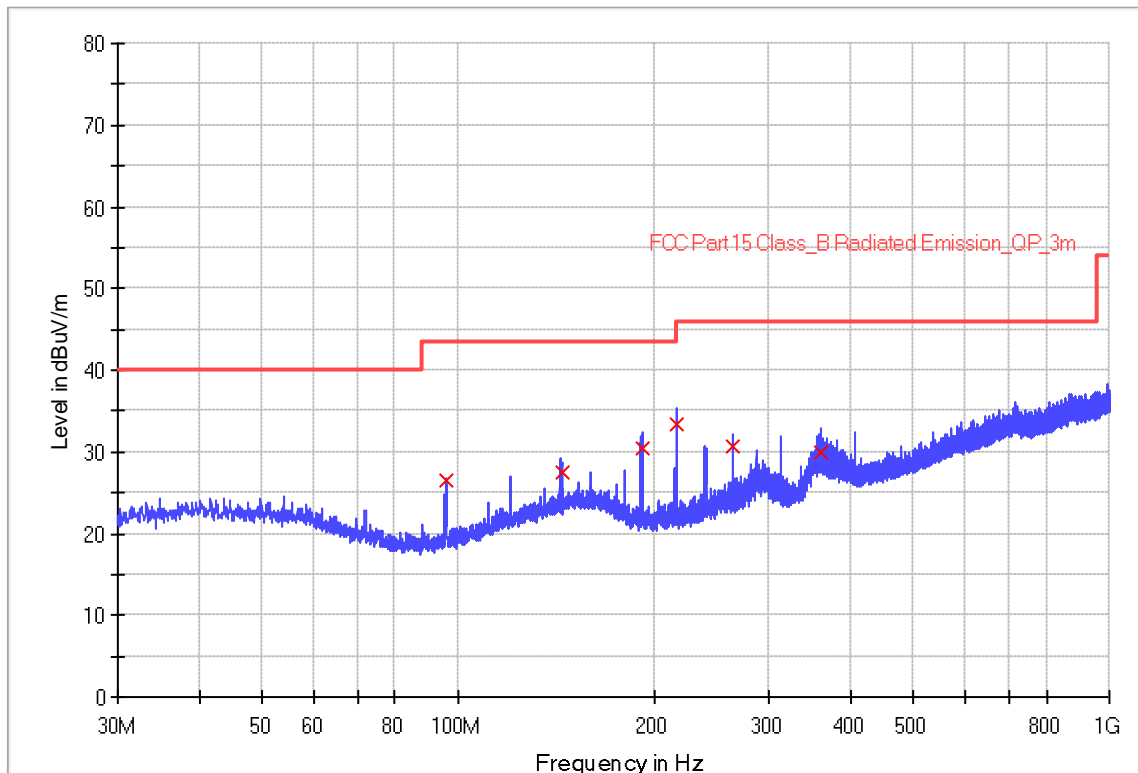
RE_VULB9168_pre_Corr_30-1000
