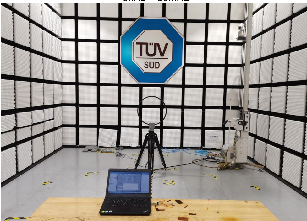
Radiated Emission Setup 9kHz ~ 30MHz
