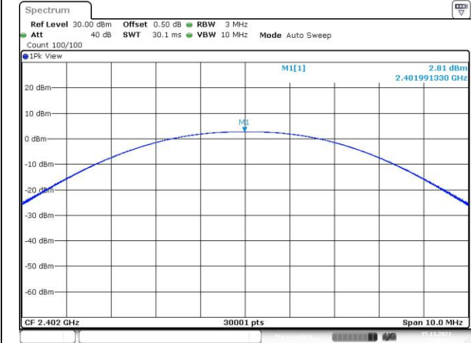
Channel 0 (2402MHz)
