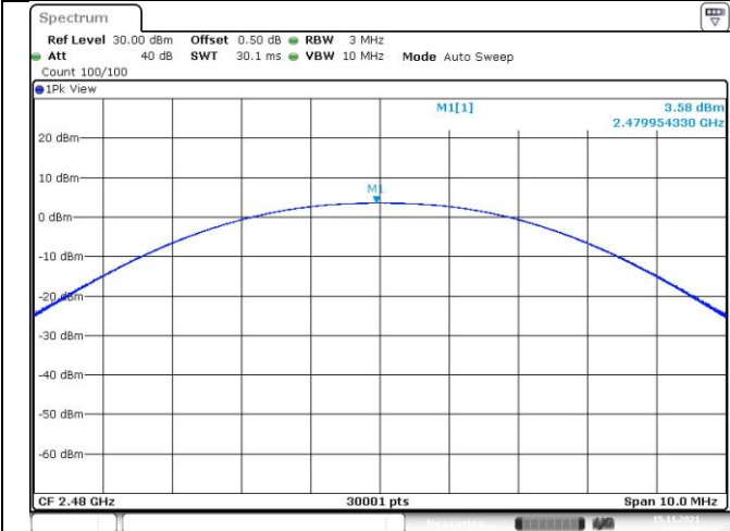
Channel 39 (2480MHz)
