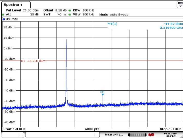
Spurious Emission (1GHz –5GHz)
