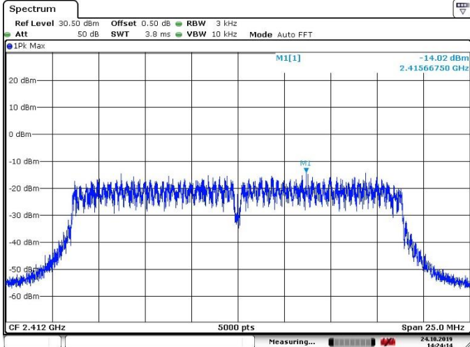
Channel 01 (2412MHz)
