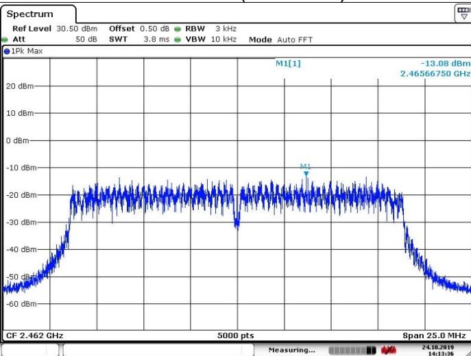
Channel 11 (2462MHz)
