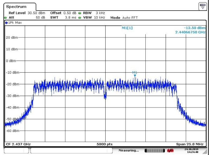
Channel 06 (2437MHz)
