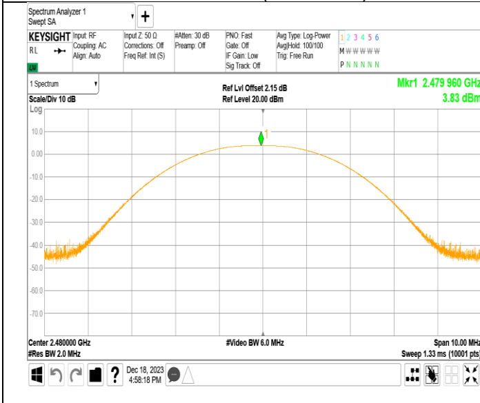
Channel 39 (2480MHz)
