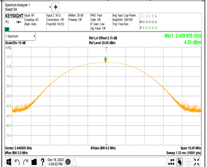
Channel 19 (2440MHz)
