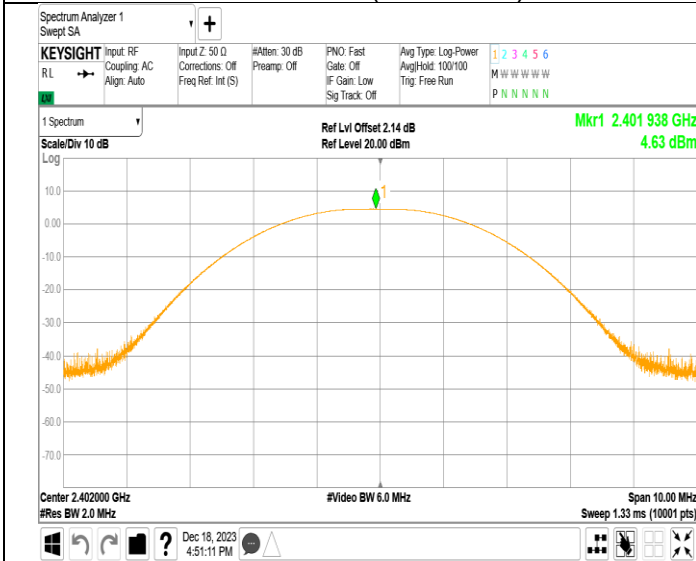
Channel 0 (2402MHz)
